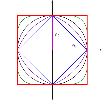
Figure 1.5: The p -balls.
