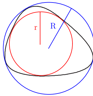
Figure 1.3: The classical inradius and circumradius.
