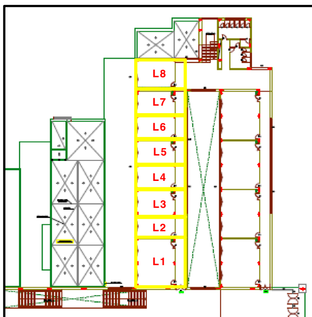
Fig. 6 Magnetic field landmarks
