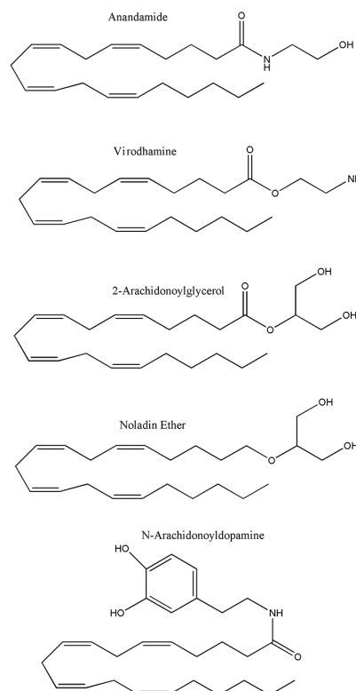
Fig. 2. Main endocannabinoids.
