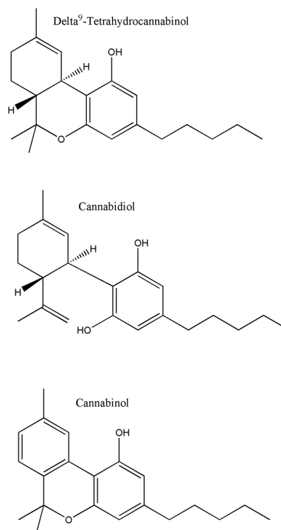
Fig. 1. Natural cannabinoids.
