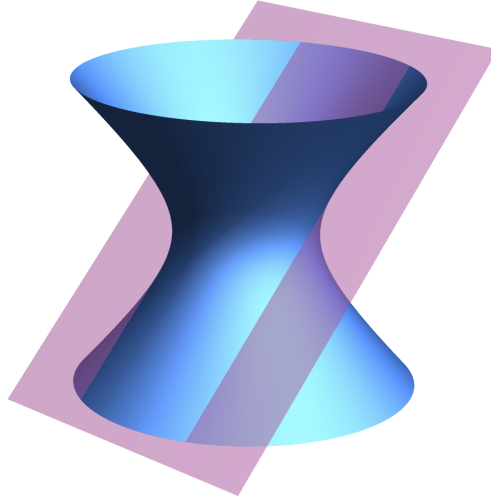
Figure 4.2: Past infinite of \mathcal{H}^{n+2}
