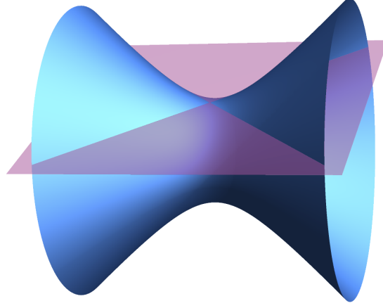
Figure 5.1: Light cone of anti-de Sitter spacetime
