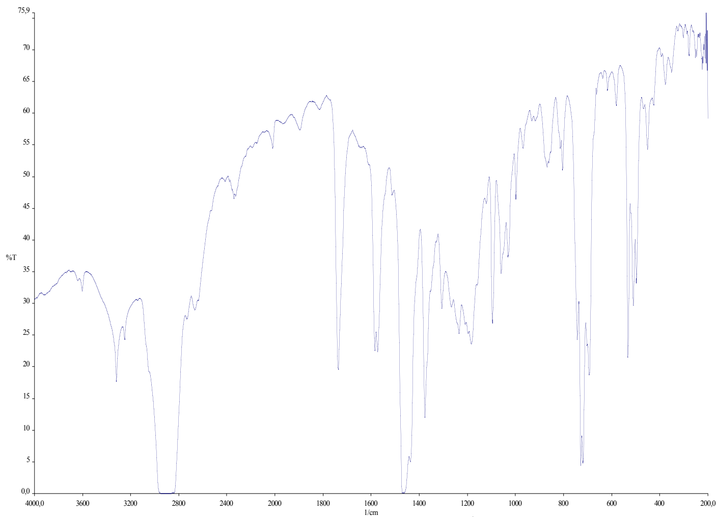
IR spectrum of 3a-Br (Nujol, \text{cm}^{-1} )
