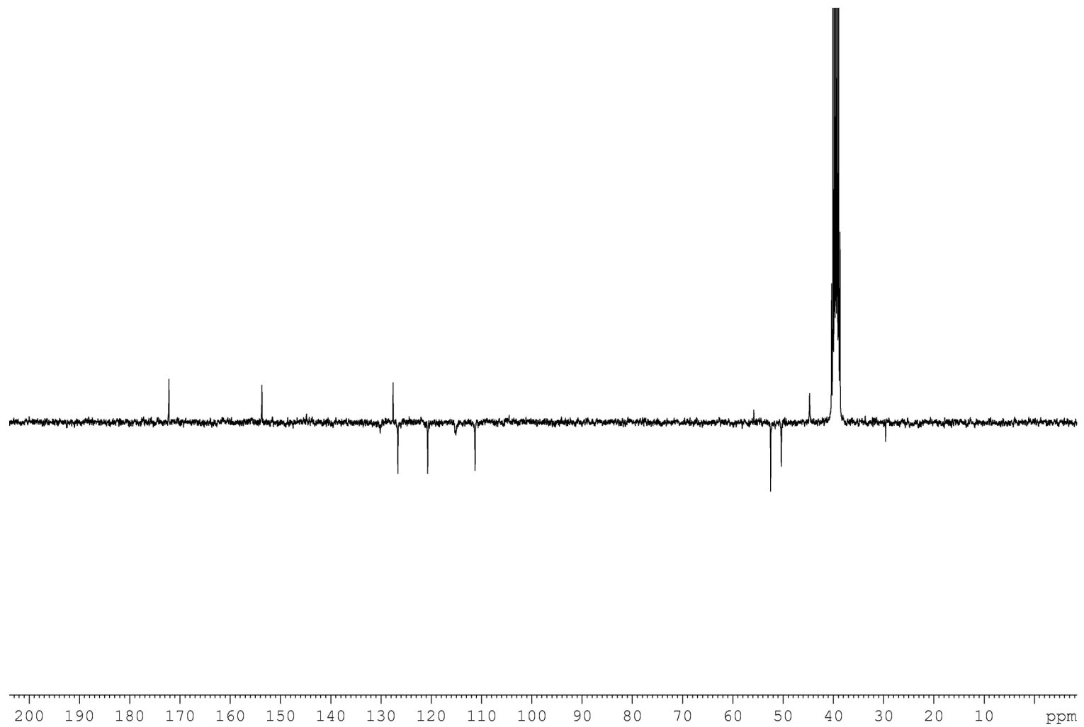
^{13}\text{C} APT NMR spectrum of 3a-Br (DMSO- d_6 , 25 °C)
