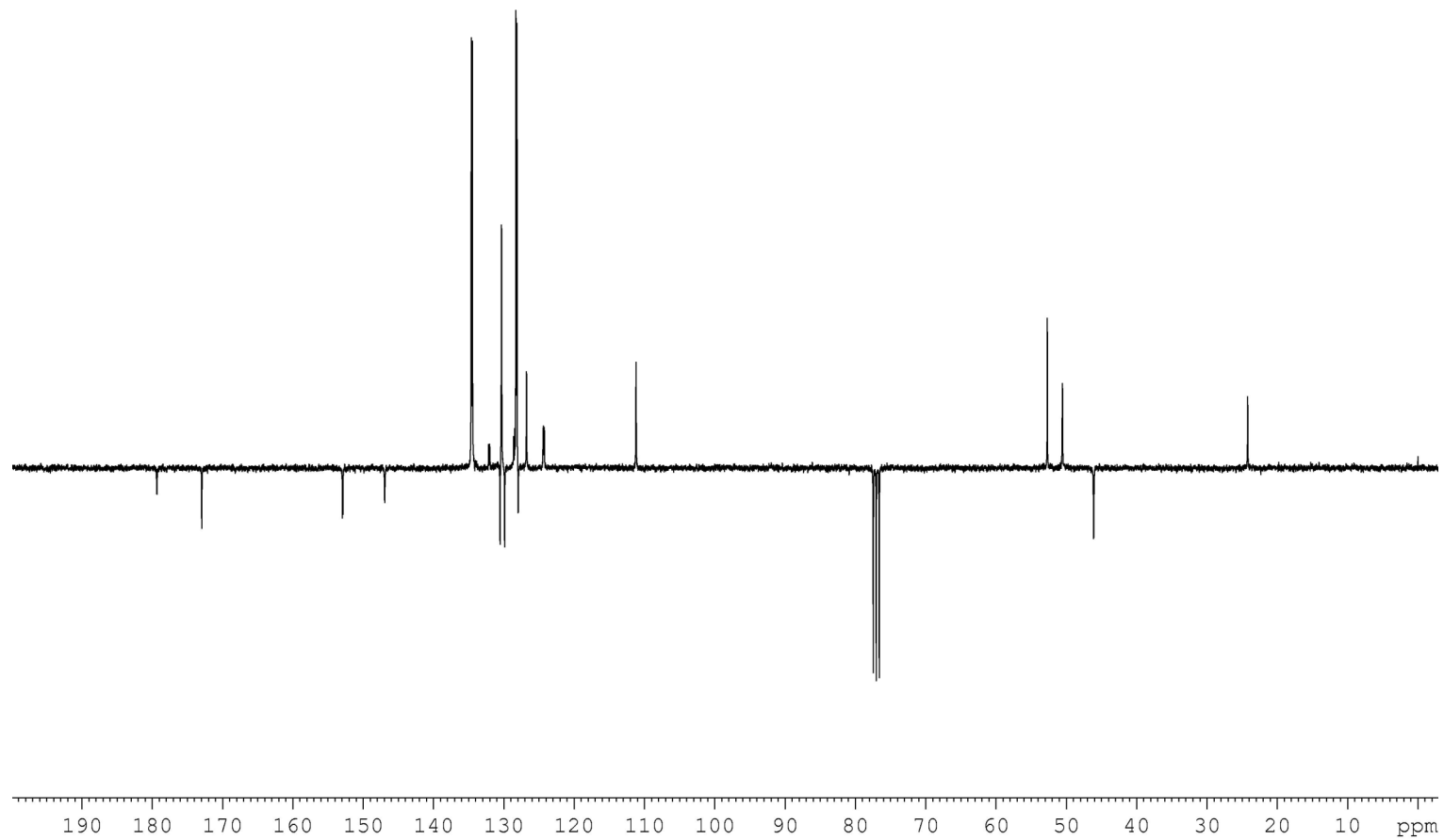
^{13}\text{C} APT NMR spectrum of 3a-OAc (CDCl 3 + TMS, 25 °C)
