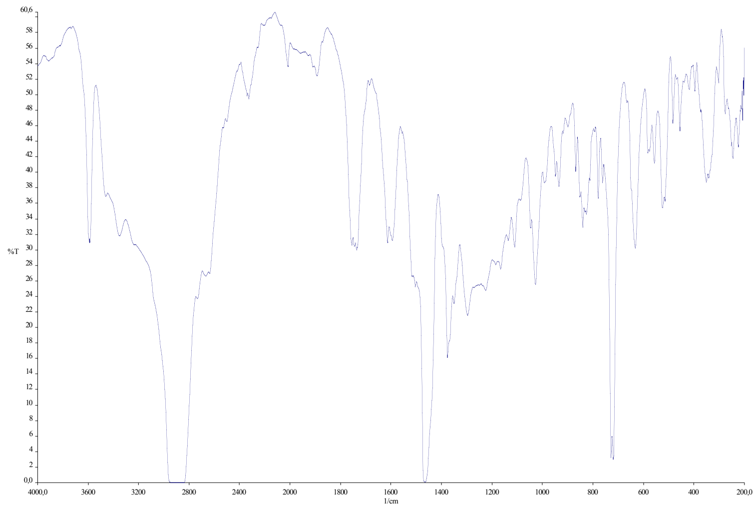
IR spectrum of A (Nujol, cm -1 )
