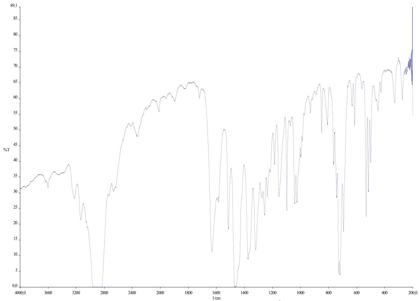
IR spectrum of 7b-OAc (Nujol, \text{cm}^{-1} )
