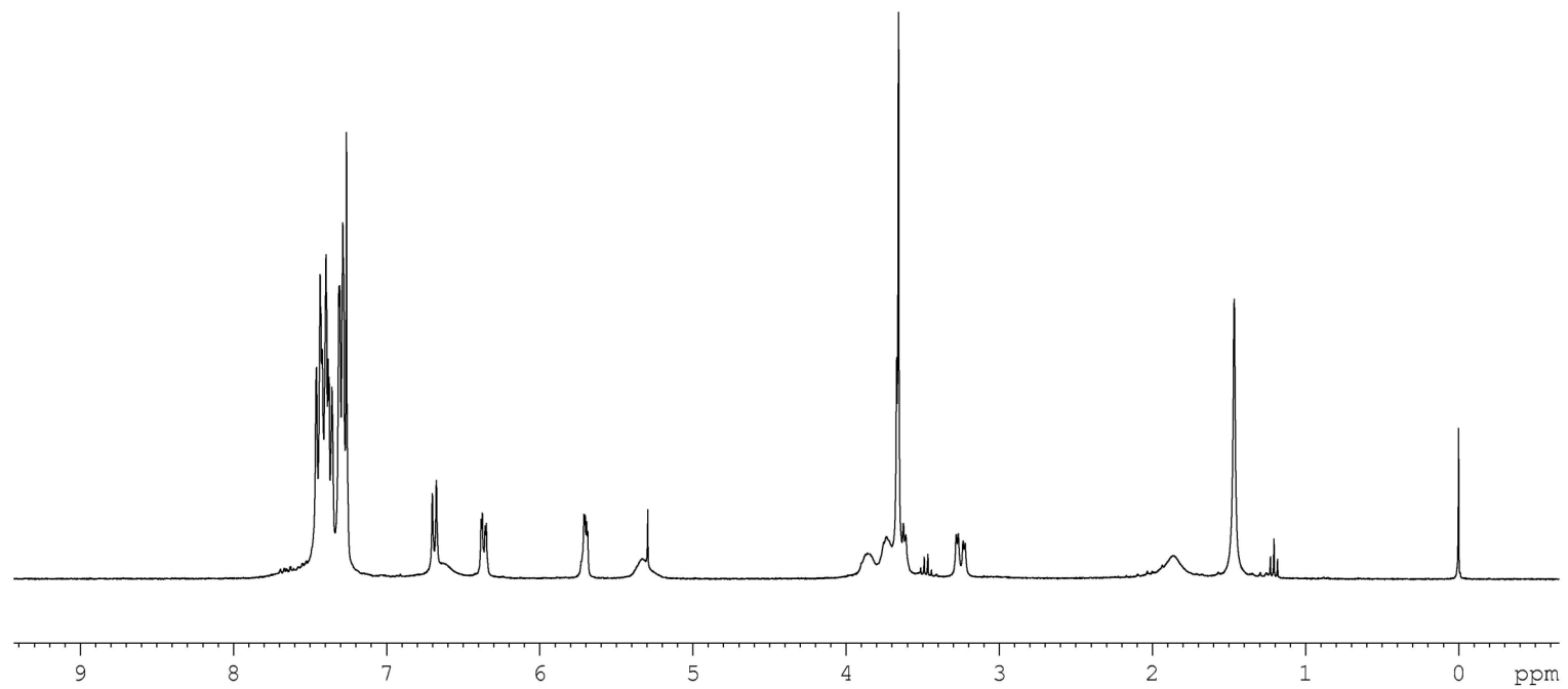
^1\text{H} NMR spectrum of 3a-OAc ( \text{CDCl}_3 + \text{TMS} , 25 °C)
