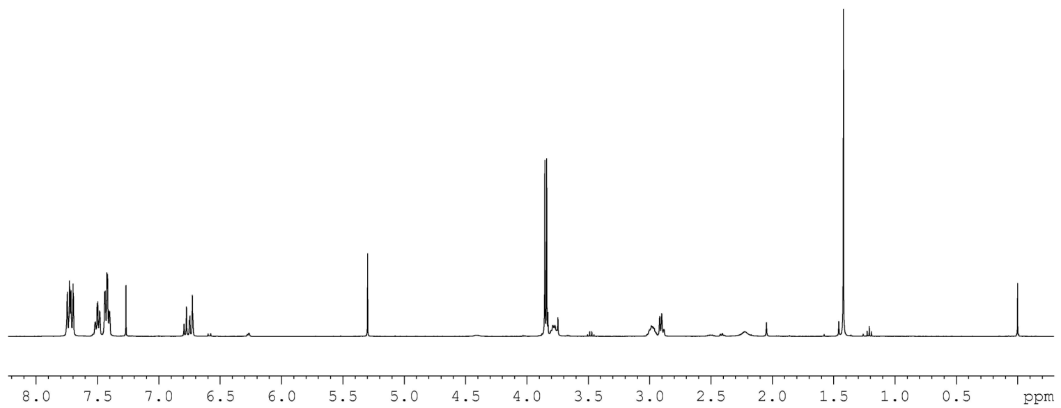
^1\text{H} NMR spectrum of 7b-OAc ( \text{CDCl}_3 + TMS, 25 °C)
