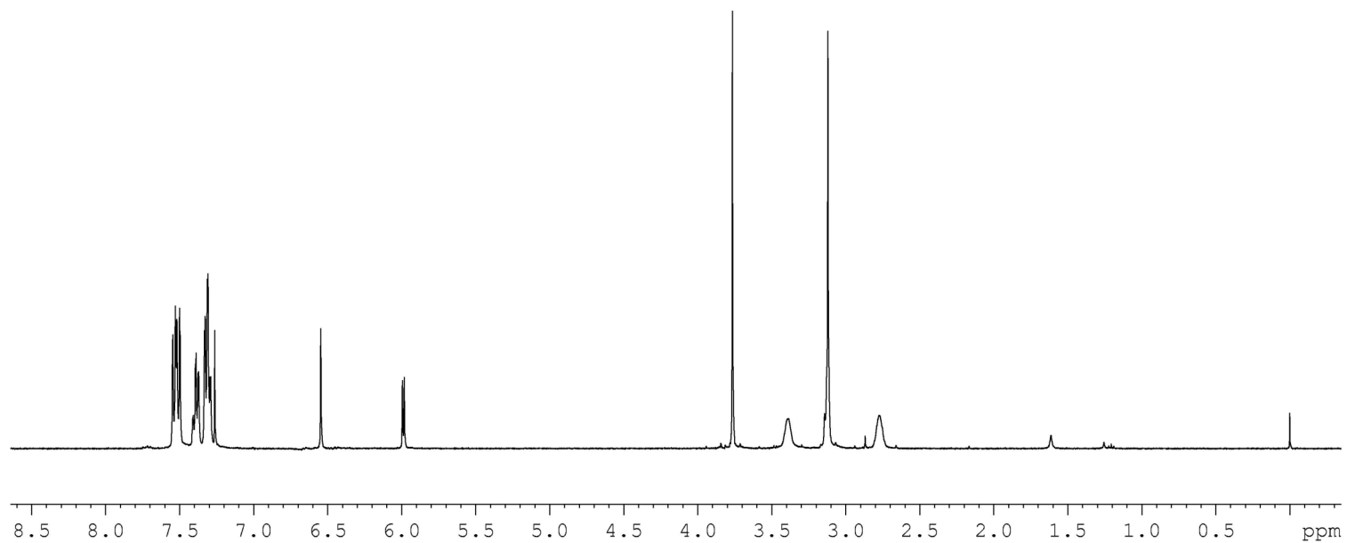
^1\text{H} NMR spectrum of 3b-Br ( \text{CDCl}_3 + TMS, 25 °C)
