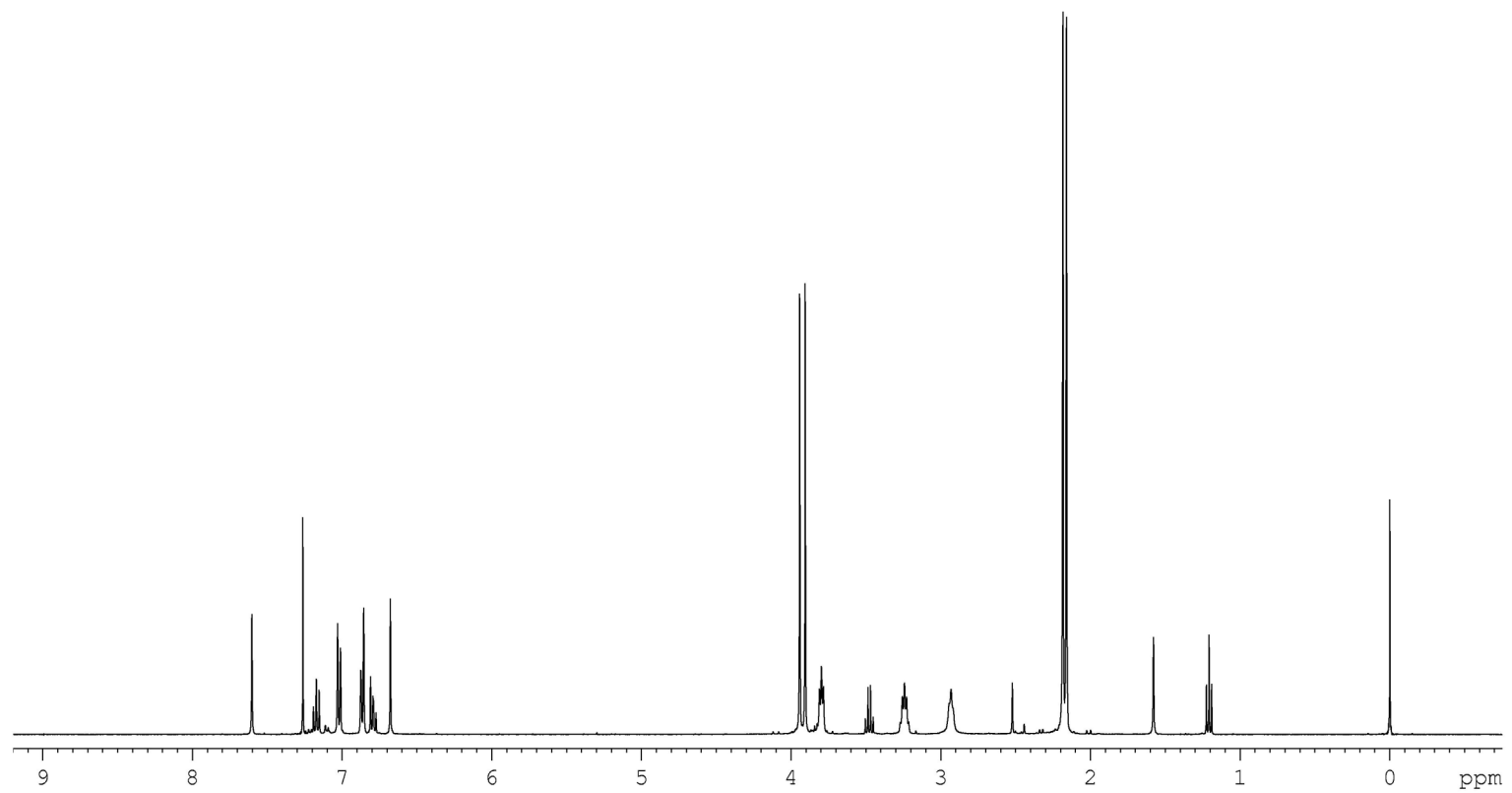
^1\text{H} NMR spectrum of 5b ( \text{CDCl}_3 + \text{TMS} , 25\text{ }^\circ\text{C} )
