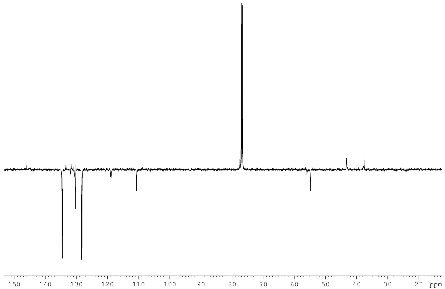
APT NMR spectrum of 3b-OAc (CDCl 3 + TMS, 25 °C)
