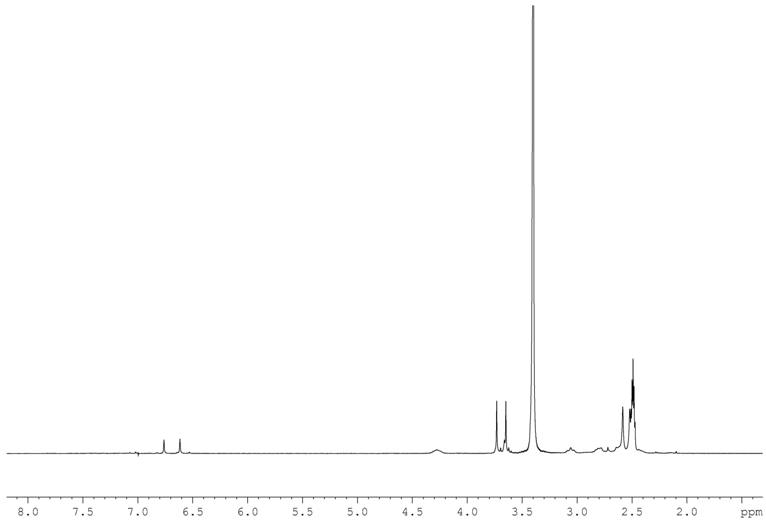
^1\text{H} NMR spectrum of 10b (DMSO- d_6 , 25 °C)
