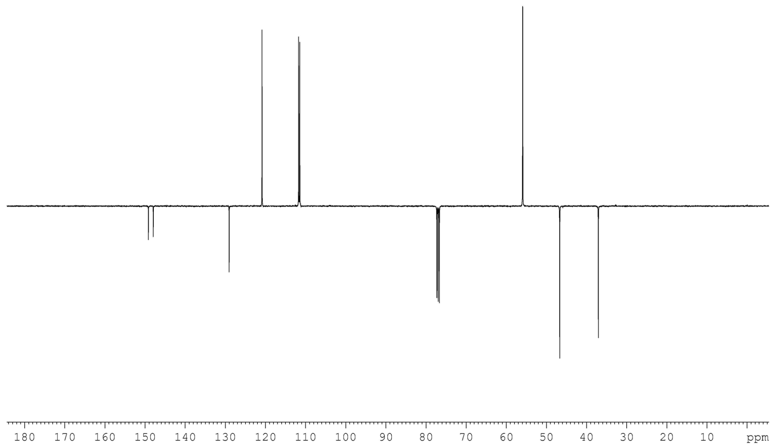
APT NMR spectrum of 6b-Br (CDCl 3 + TMS, 25 °C)
