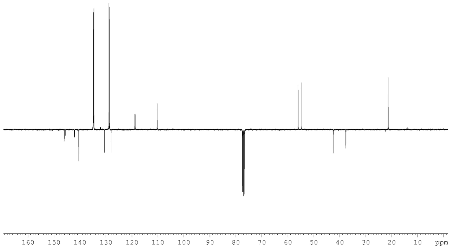
APT NMR spectrum of 3'b-Br (CDCl 3 + TMS, 25 °C)
