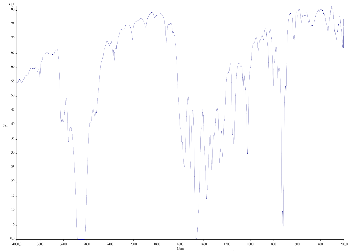
IR spectrum of 6b-OAc (Nujol, cm -1 )
