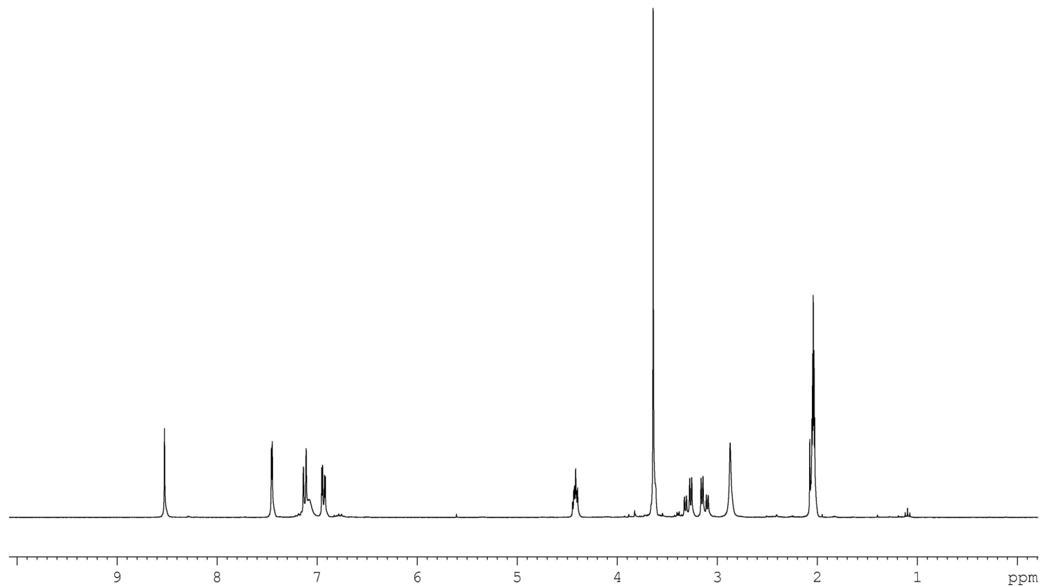
^1\text{H} NMR spectrum of 10a (acetone- d_6 , 25 °C)
