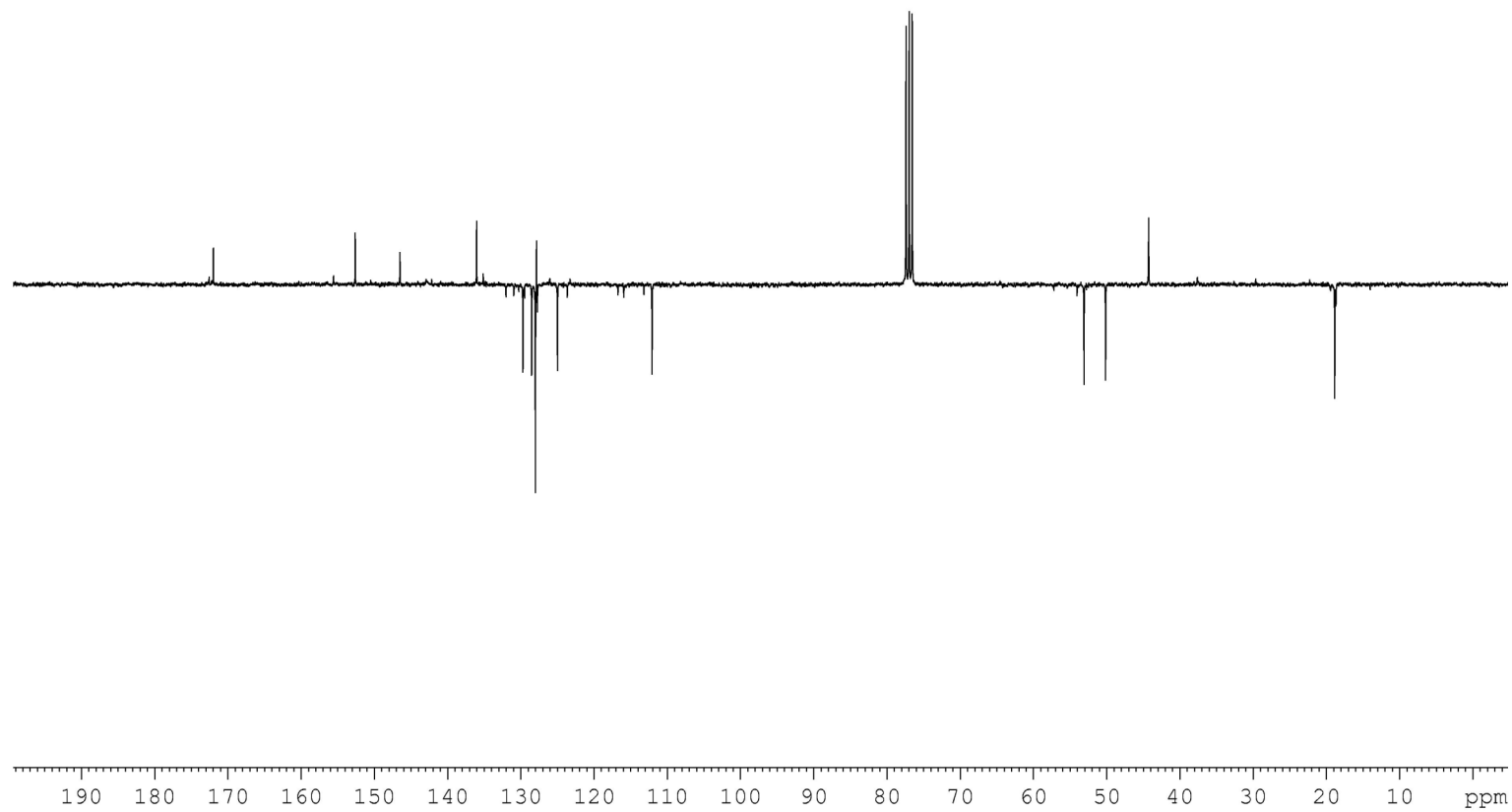
^{13}\text{C} APT NMR spectrum of 4a ( \text{CDCl}_3 + TMS, 25 °C)
