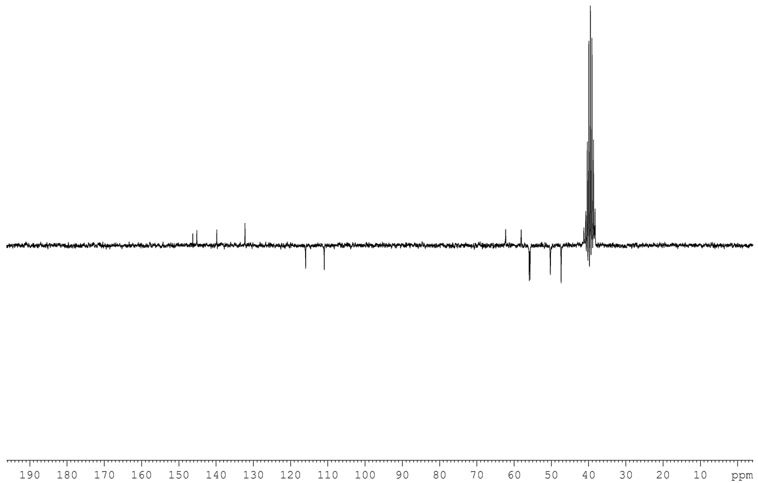
APT NMR spectrum of 9b (DMSO- d 6 , 25 °C)
