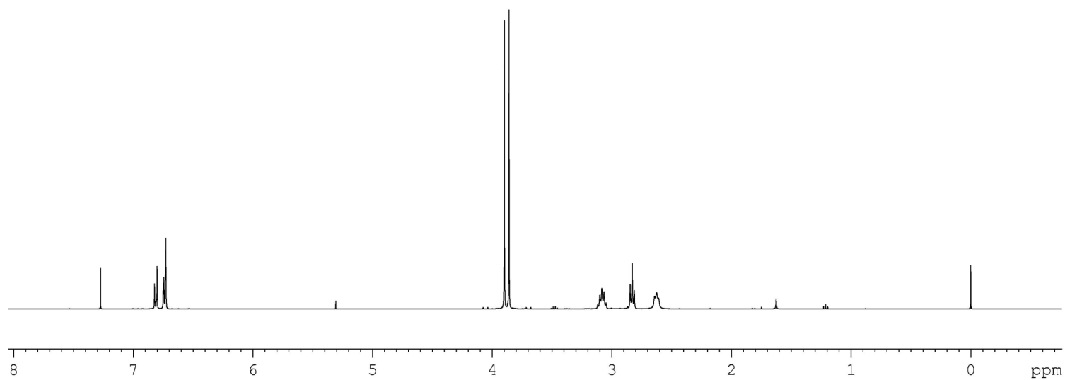
^1\text{H} NMR spectrum of 6b-Br ( \text{CDCl}_3 + TMS, 25 °C)
