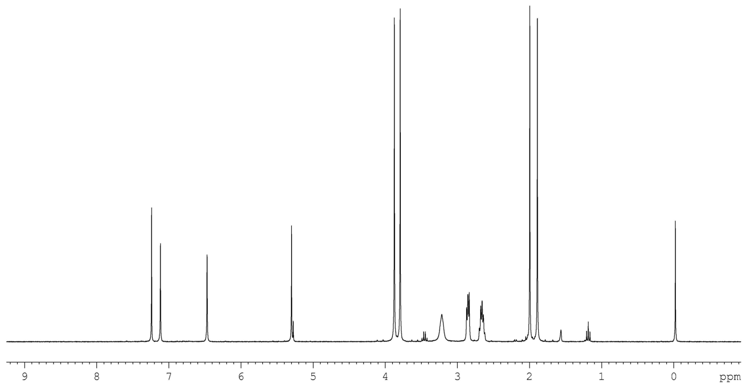
^1\text{H} NMR spectrum of 2b ( \text{CDCl}_3 + \text{TMS} , 25\text{ }^\circ\text{C} )
