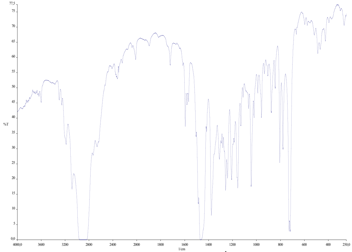
IR spectrum of 9b (Nujol, cm -1 )
