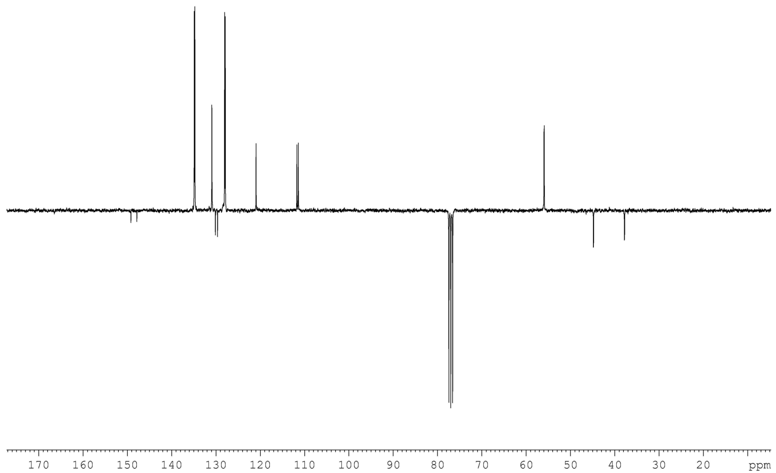
APT NMR spectrum of 7b-Br (CDCl 3 + TMS, 25 °C)
