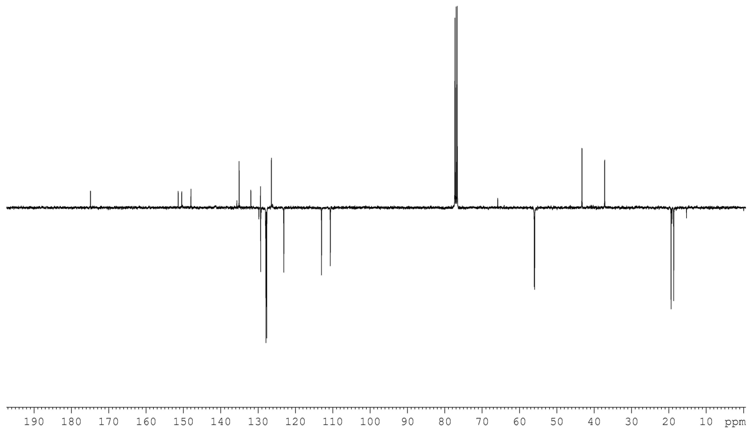
APT NMR spectrum of 5b (CDCl 3 + TMS, 25 °C)
