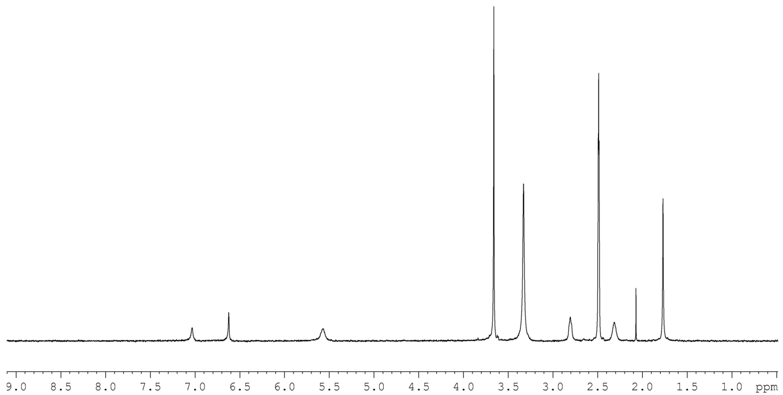
^1\text{H} NMR spectrum of 1b-OAc (DMSO- d_6 , 25 °C)
