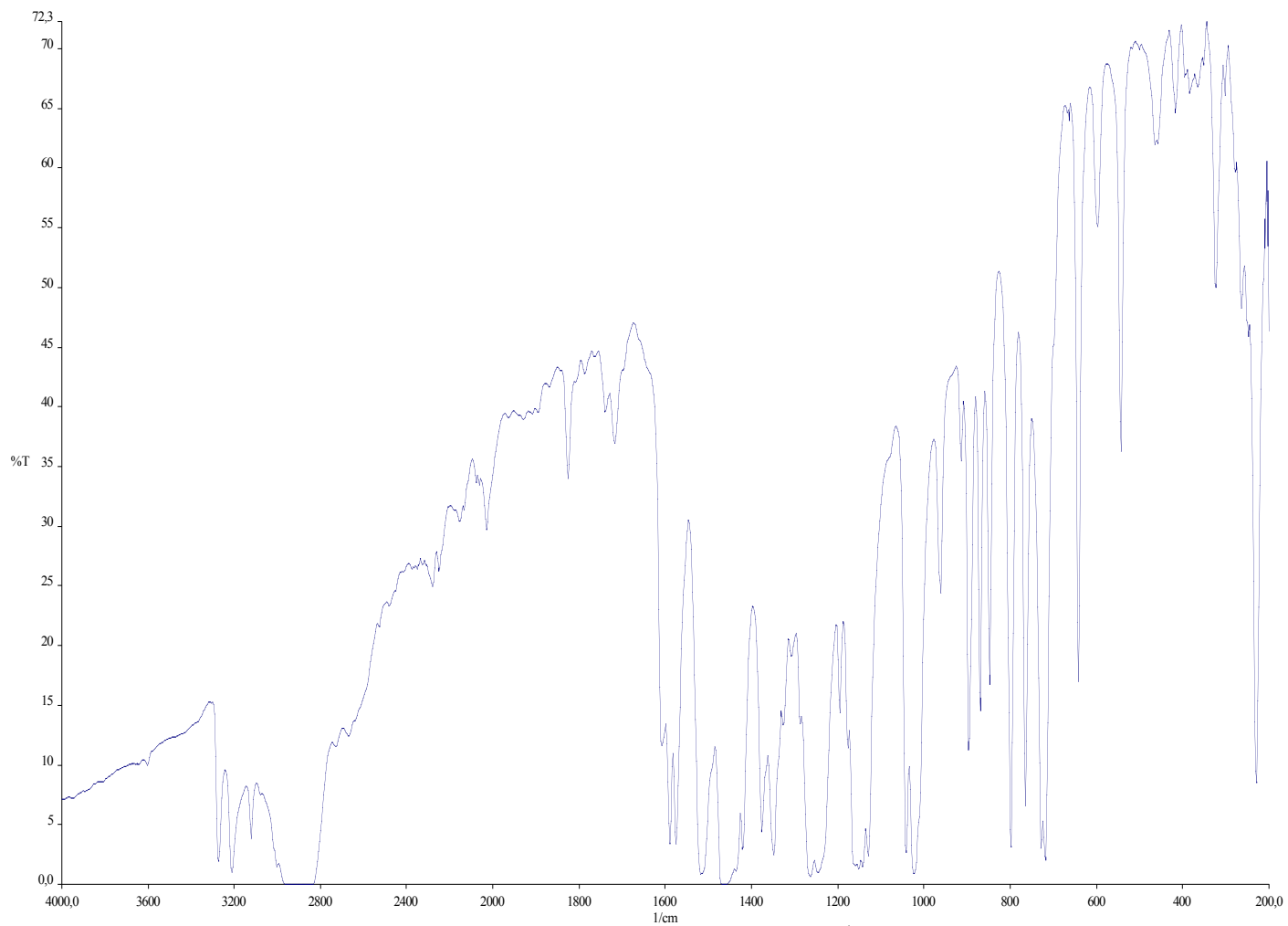
IR spectrum of 6b-Br (Nujol, cm -1 )
