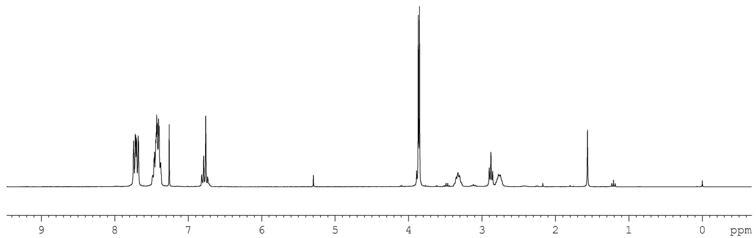
^1\text{H} NMR spectrum of 7b-Br ( \text{CDCl}_3 + TMS, 25 °C)
