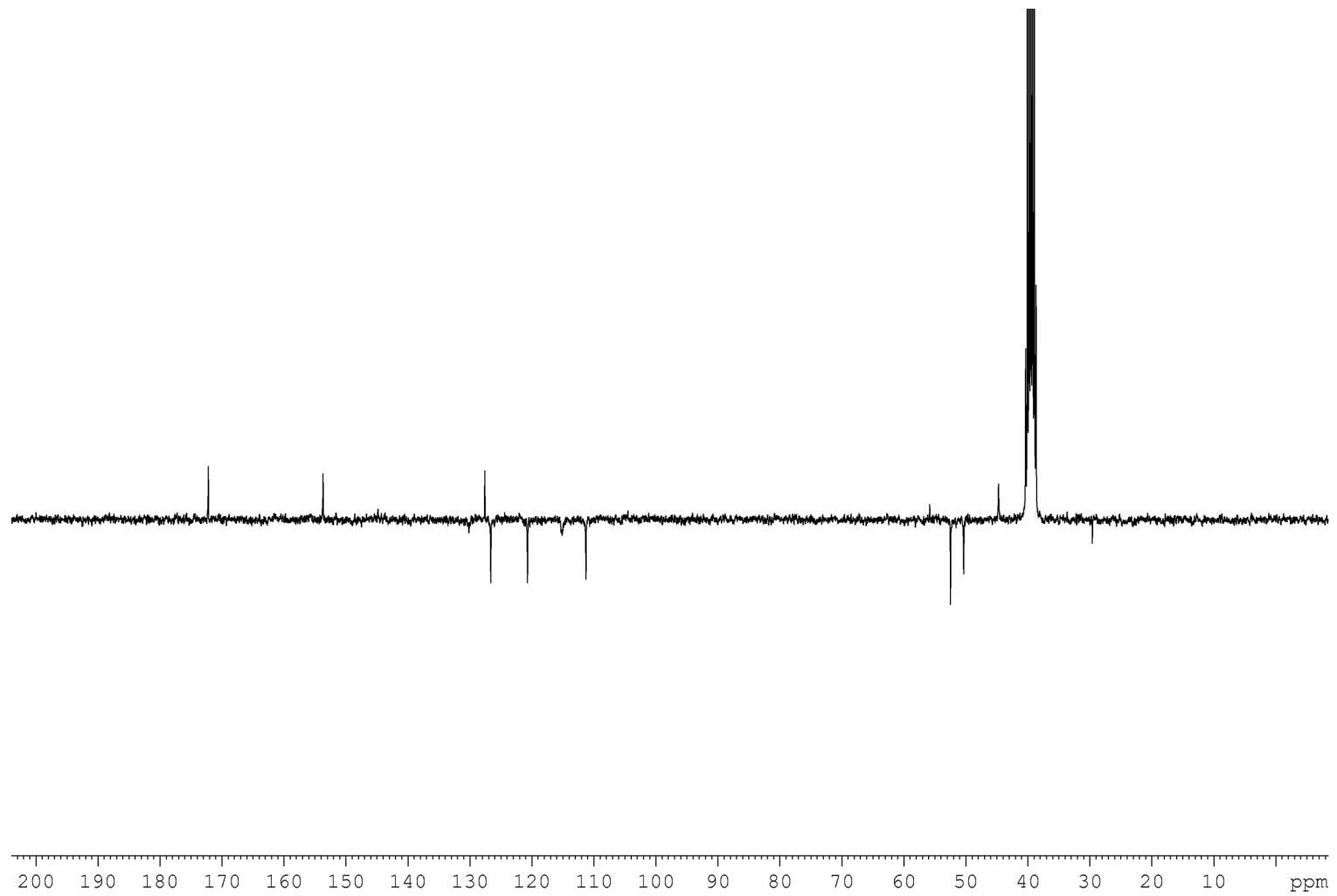
^{13}\text{C} APT NMR spectrum of 1a-OAc (DMSO- d_6 , 25 °C)
