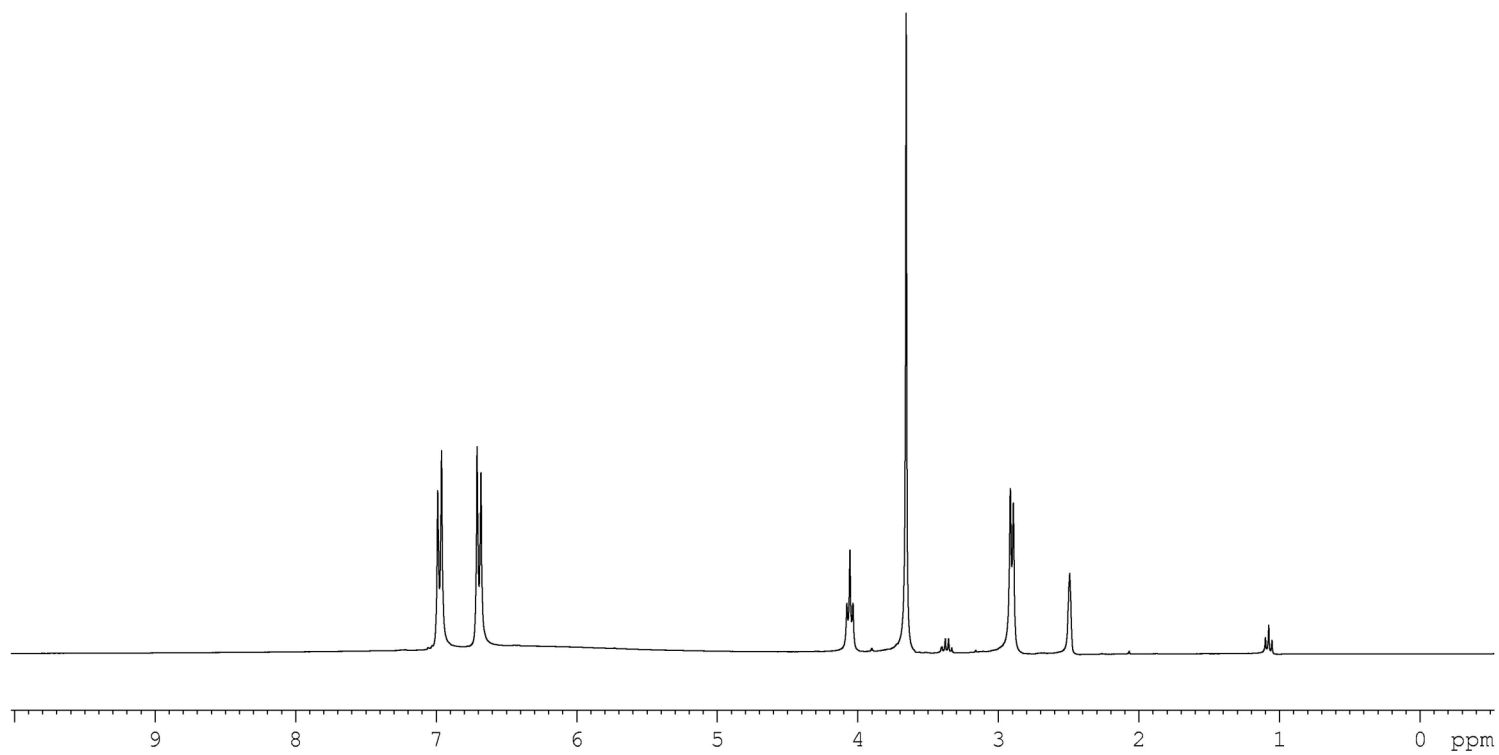
^1\text{H} NMR spectrum of A (DMSO- d_6 , 25 °C)
