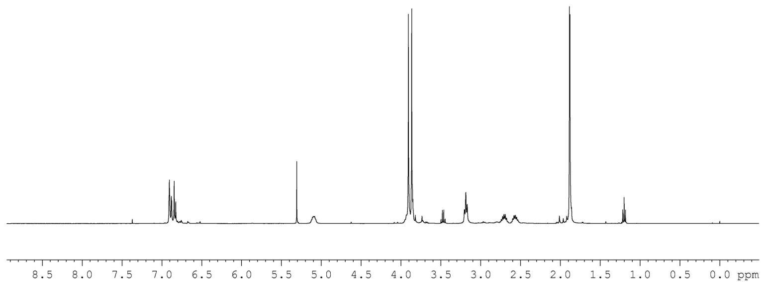
^1\text{H} NMR spectrum of 8b ( \text{CDCl}_3 + \text{TMS} , 25 °C)
