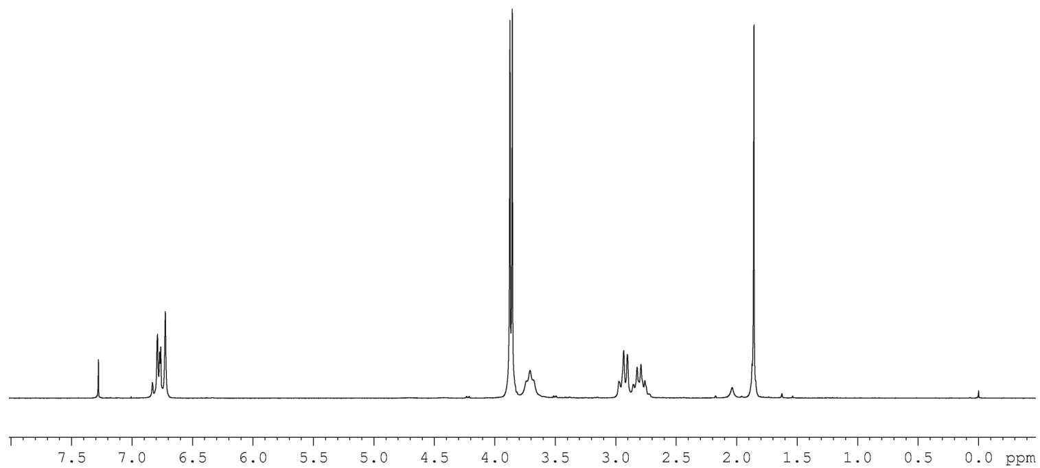
^1\text{H} NMR spectrum of 6b-OAc (CDCl 3 + TMS, 25 °C)
