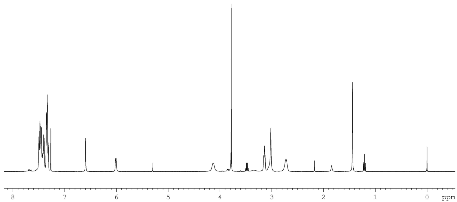
^1\text{H} NMR spectrum of 3b-OAc ( \text{CDCl}_3 + TMS, 25 °C)
