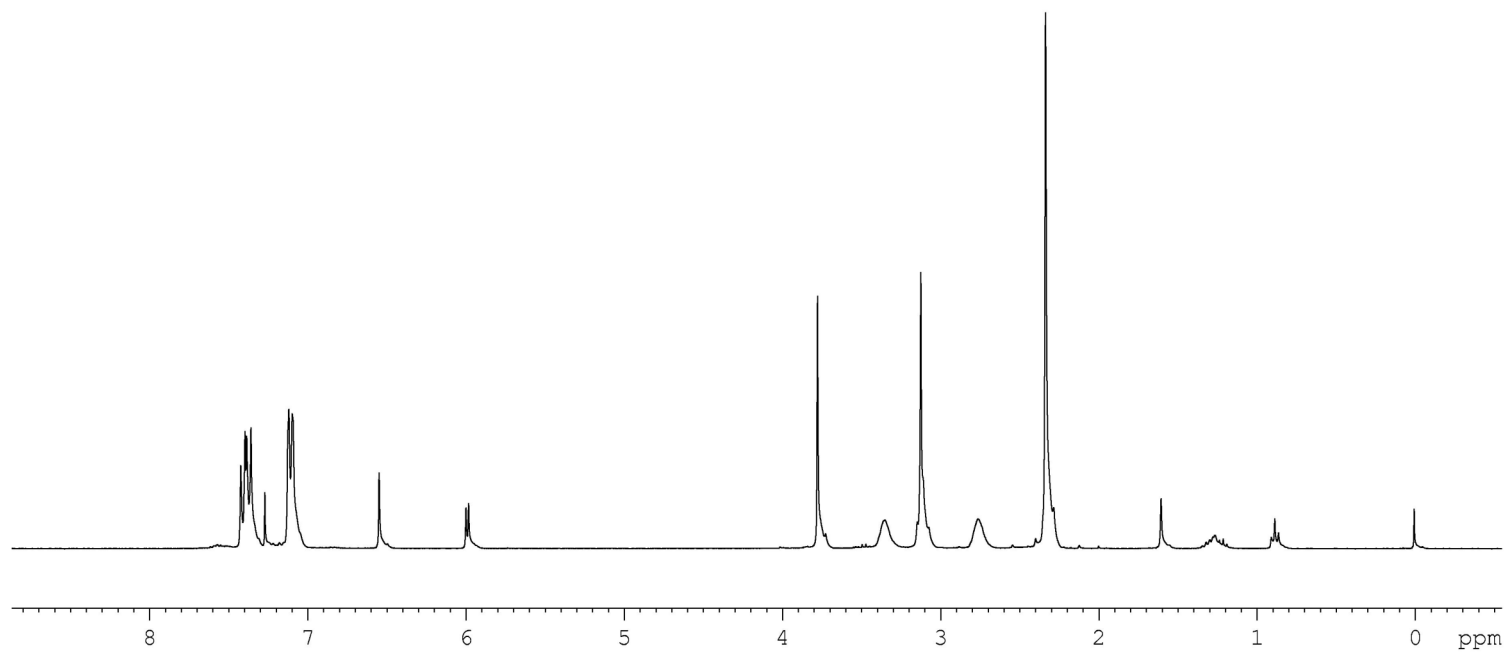
^1\text{H} NMR spectrum of 3'b-Br (CDCl 3 + TMS, 25 °C)
