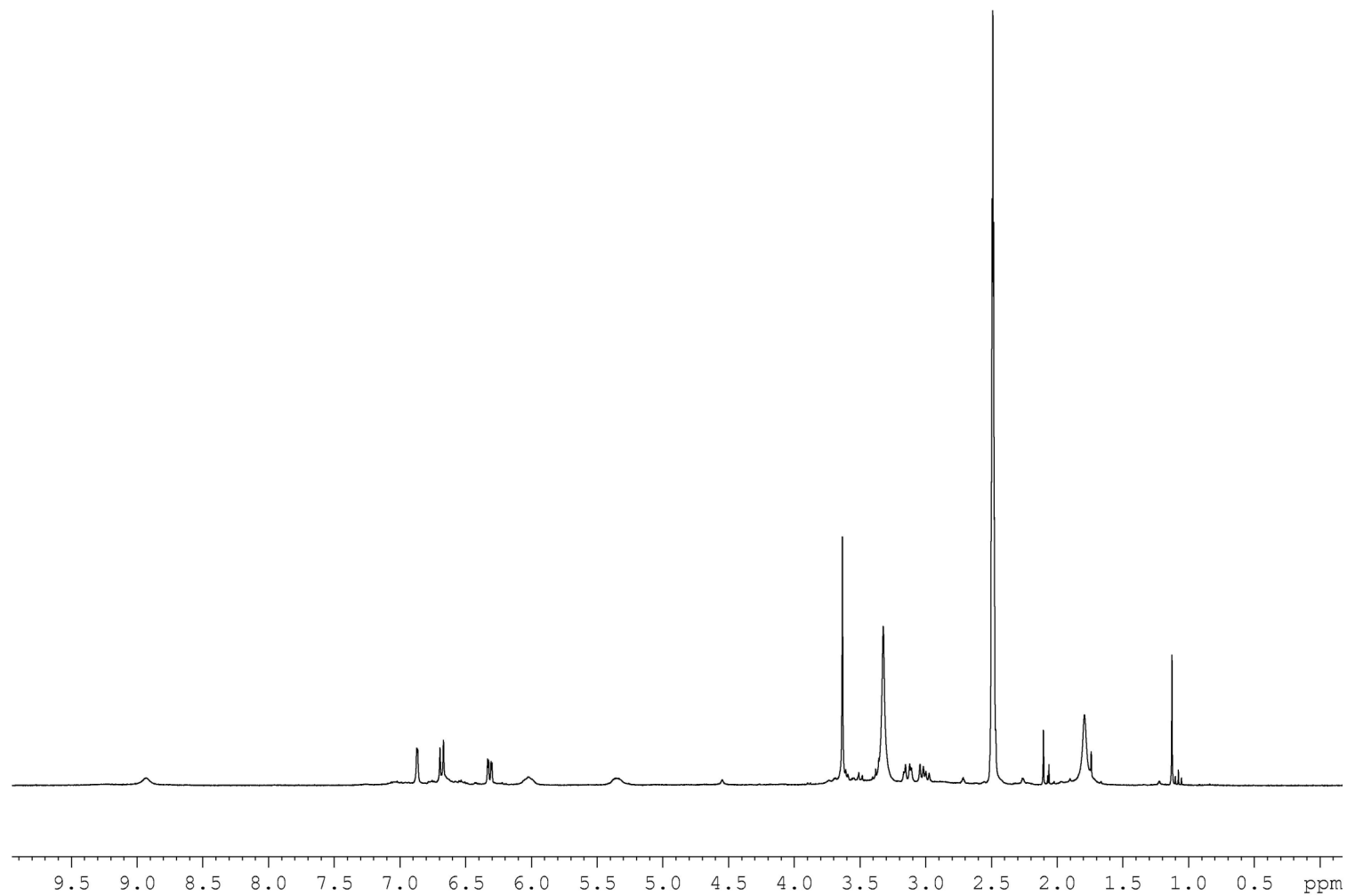
^1\text{H} NMR spectrum of 1a-OAc (DMSO- d_6 , 25 °C)
