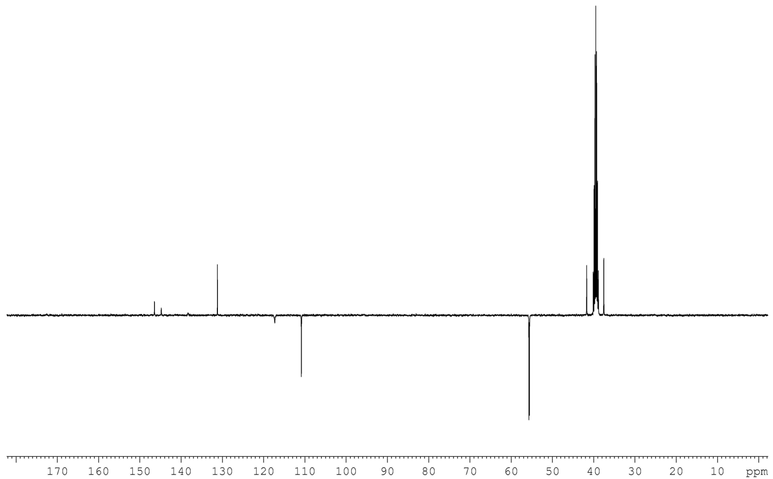
^{13}\text{C} APT NMR spectrum of 1b-Br (DMSO- d_6 , 25 °C)
