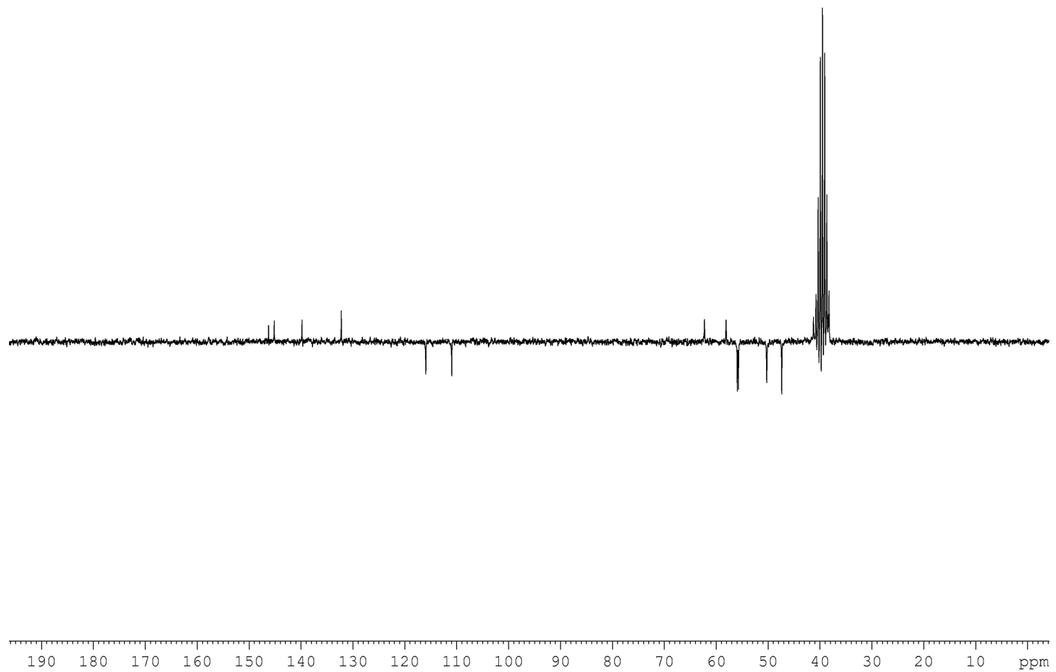
APT NMR spectrum of 10b (DMSO- d_6 , 25 °C)
