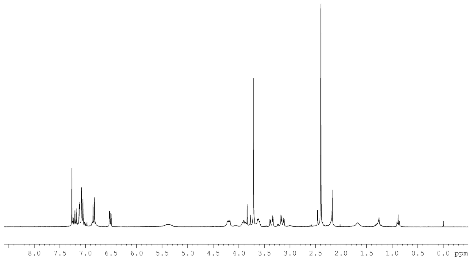
^1\text{H} NMR spectrum of 4a ( \text{CDCl}_3 + \text{TMS} , 25 °C)
