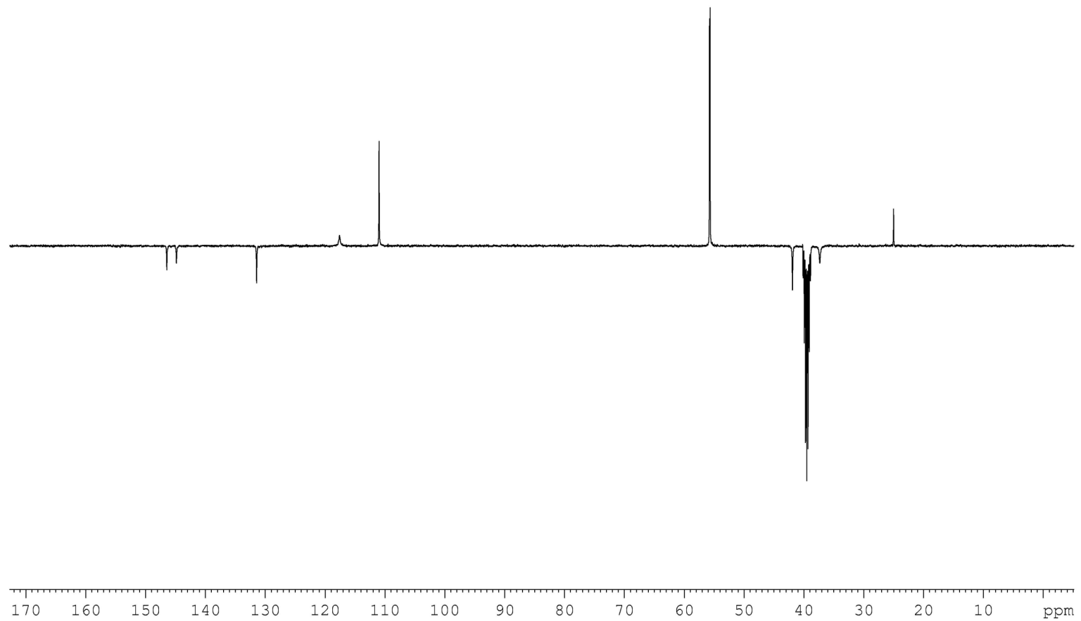
^{13}\text{C} APT NMR spectrum of 1b-OAc ( \text{DMSO-}d_6 , 25\text{ }^\circ\text{C} )
