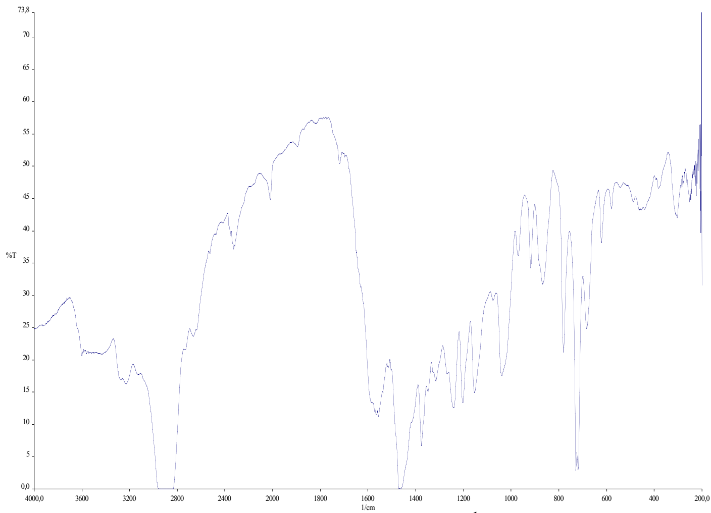
IR spectrum of 1b-OAc (Nujol, cm -1 )
