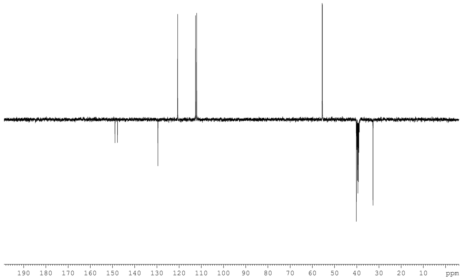
^{13}\text{C} APT NMR spectrum of B ( \text{DMSO-}d_6 , 25\text{ }^\circ\text{C} )
