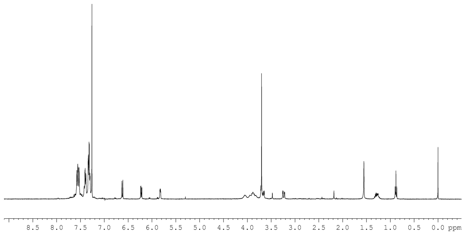
^1\text{H} NMR spectrum of 3a-Br
