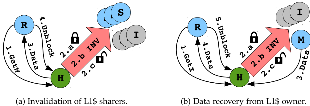
Figure 5.3: Examples of coherence scenarios under the baseline ECONO protocol.
