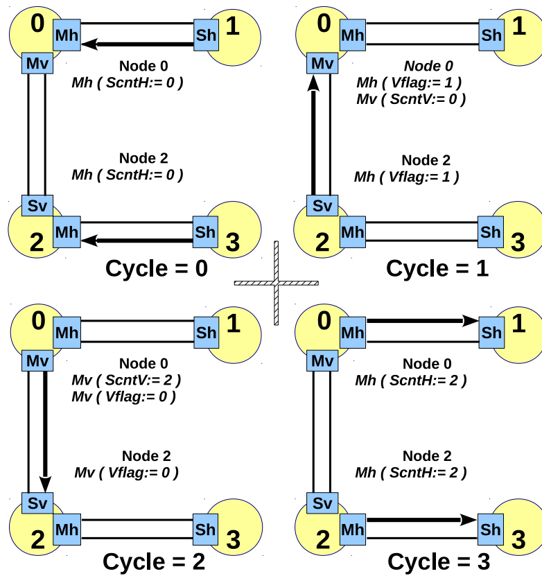
Figure 3.4: Barrier synchronization under GBarrier .
