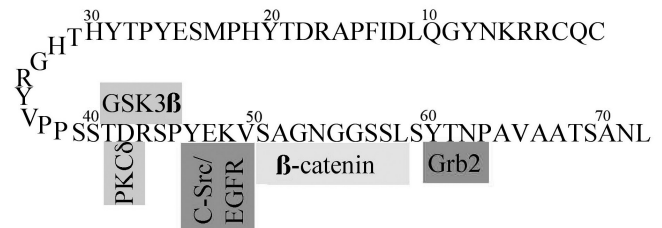
Fig. 1. MUC1 cytoplasmic tail signaling. MUC1 cytoplasmic tail can be phosphorylated on i) Ser 44 by GSK3 \beta binding to TDRSP, ii) Tyr 46 by c-Src or EGFR binding to YEKV, iii) Thr 41 by PKC \delta binding to TDR and iv) Tyr 60 by Grb2 binding to YTNP. In addition, the phosphorylation at Tyr 46 and Thr 41 enhances the binding of \beta -catenin to SAGNGGSSLS of MUC1 cytoplasmic region.
