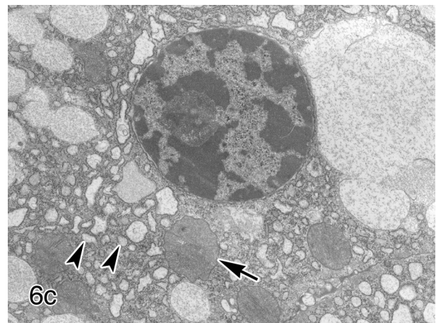
Fig. 6. Electron micrographs of submandibular gland parenchyma. a. Reperfusion time 1 day after 3-h ligation time. Granular duct with a cell (arrow) showing apoptotic features. x 900. b. Higher magnification of arrowed portion in a. x 5000. c. Reperfusion time 1 day after 6-h ligation time. Acinar cell showing necrotic features. Swelling of the mitochondria (arrow) and integration of rER (arrowhead) can be seen. x 10,000
