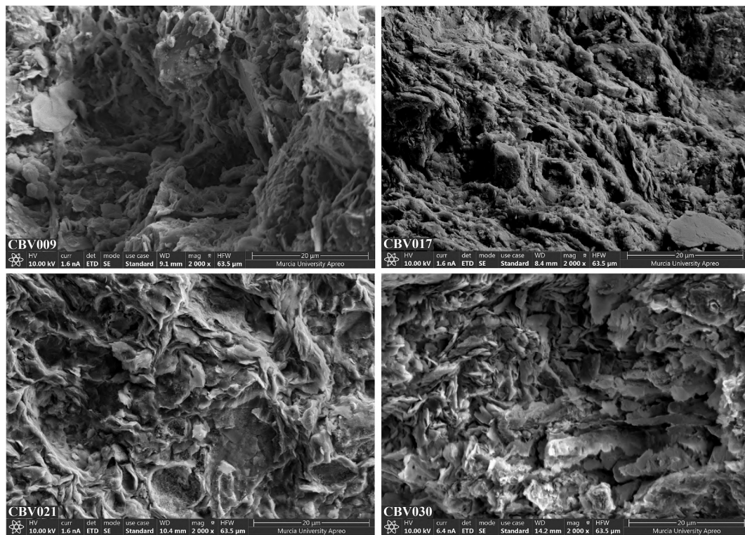
Fig. 5. SEM photomicrographs showing the ‘no vitrification’ stage in individuals from Cobatillas la Vieja: (A) CBV009 (CBV-F4, XRD group 4.1); (B) CBV017 (CBV-F1, XRD group 1); (C) CBV021 (CBV-F3, XRD group 3.2); (D) CBV030 (CBV-F2, XRD group 2.1).
