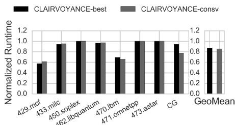
Fig. 11: Normalized runtime w.r.t. original execution (-O3) for Clairvoyance-consv (with better alias analysis and heuristic to choose between hoisting and prefetching) and the previous Clairvoyance-best.
