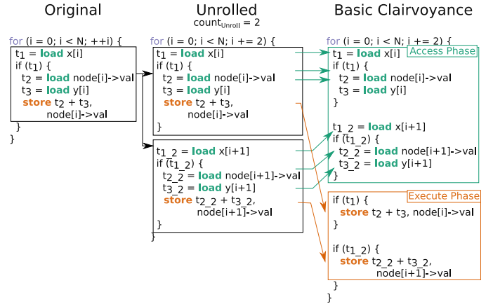
Fig. 1: The basic Clairvoyance transformation. The original loop is first unrolled by count unroll which increases the number of instructions per loop iteration. Then, for each iteration, Clairvoyance hoists all (critical) loads and sinks their uses to create a memory-bound Access phase and a compute-bound Execute phase.
