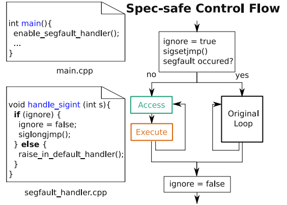
Fig. 4: Custom segmentation fault handler to safely execute spec-safe. The handler is deployed at program start (left, main.cpp ). On a segmentation fault, the handler will either (1) raise the fault in the default handler, or (2) re-execute the original loop (left, segfault_handler.cpp , jump to sigsetjmp ). The decision depends on a flag ( ignore ).
