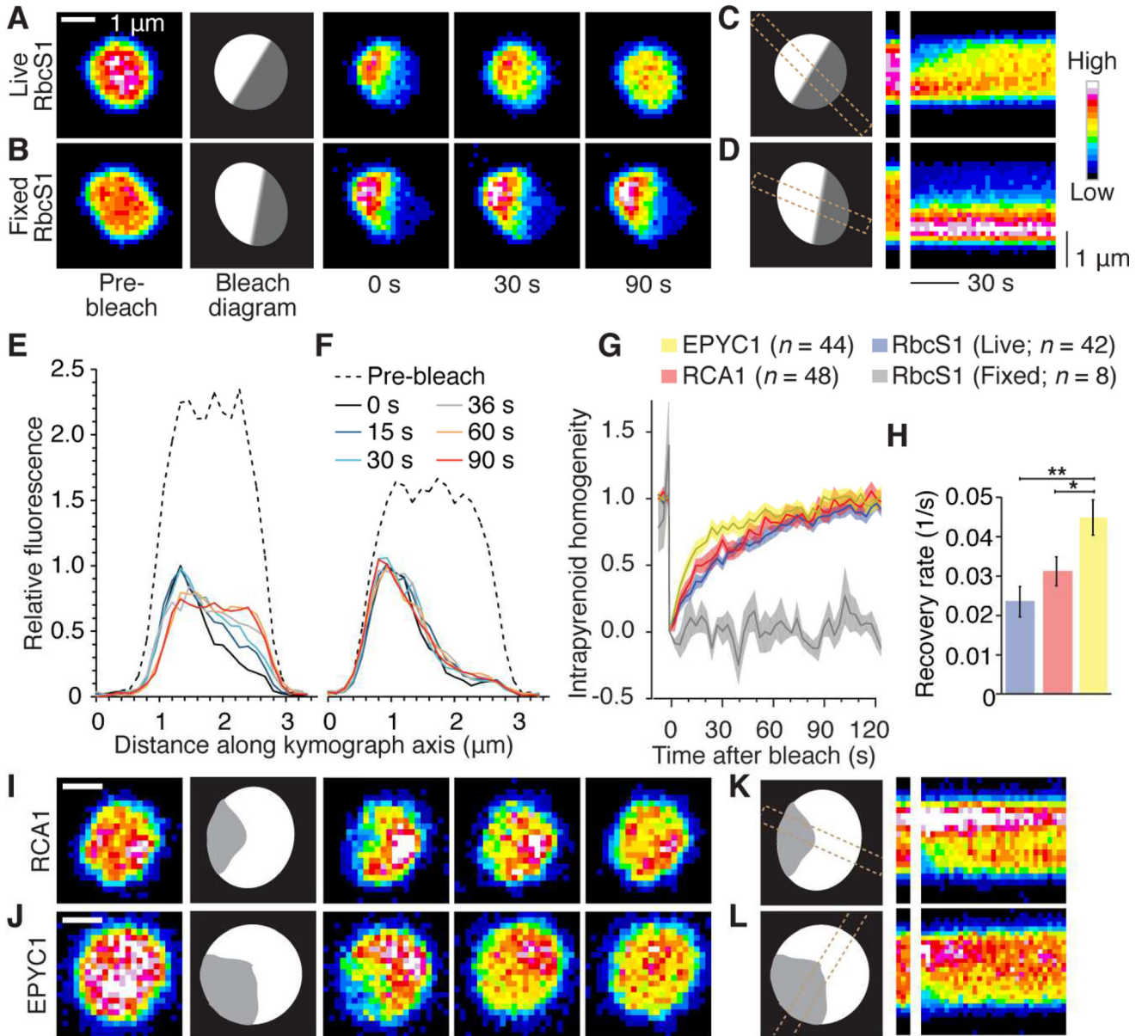
Figure 5. Pyrenoid Matrix Components Mix Internally
