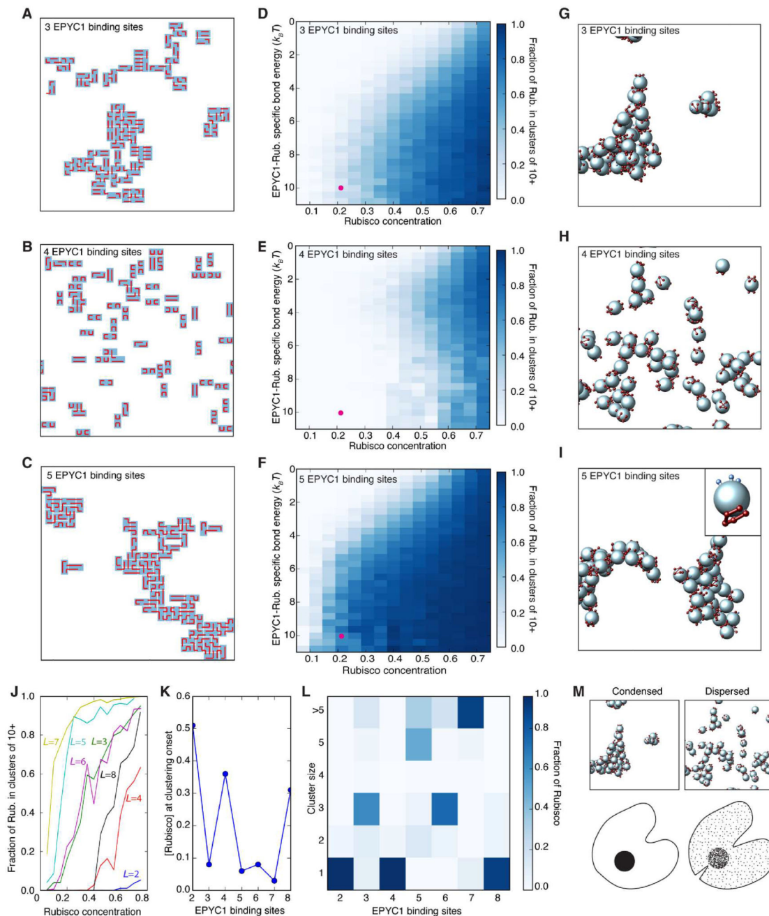
Figure 7. Simulations of an EPYC1-Rubisco System Reveal an Effect of Binding Site Stoichiometry on the Aggregation State
