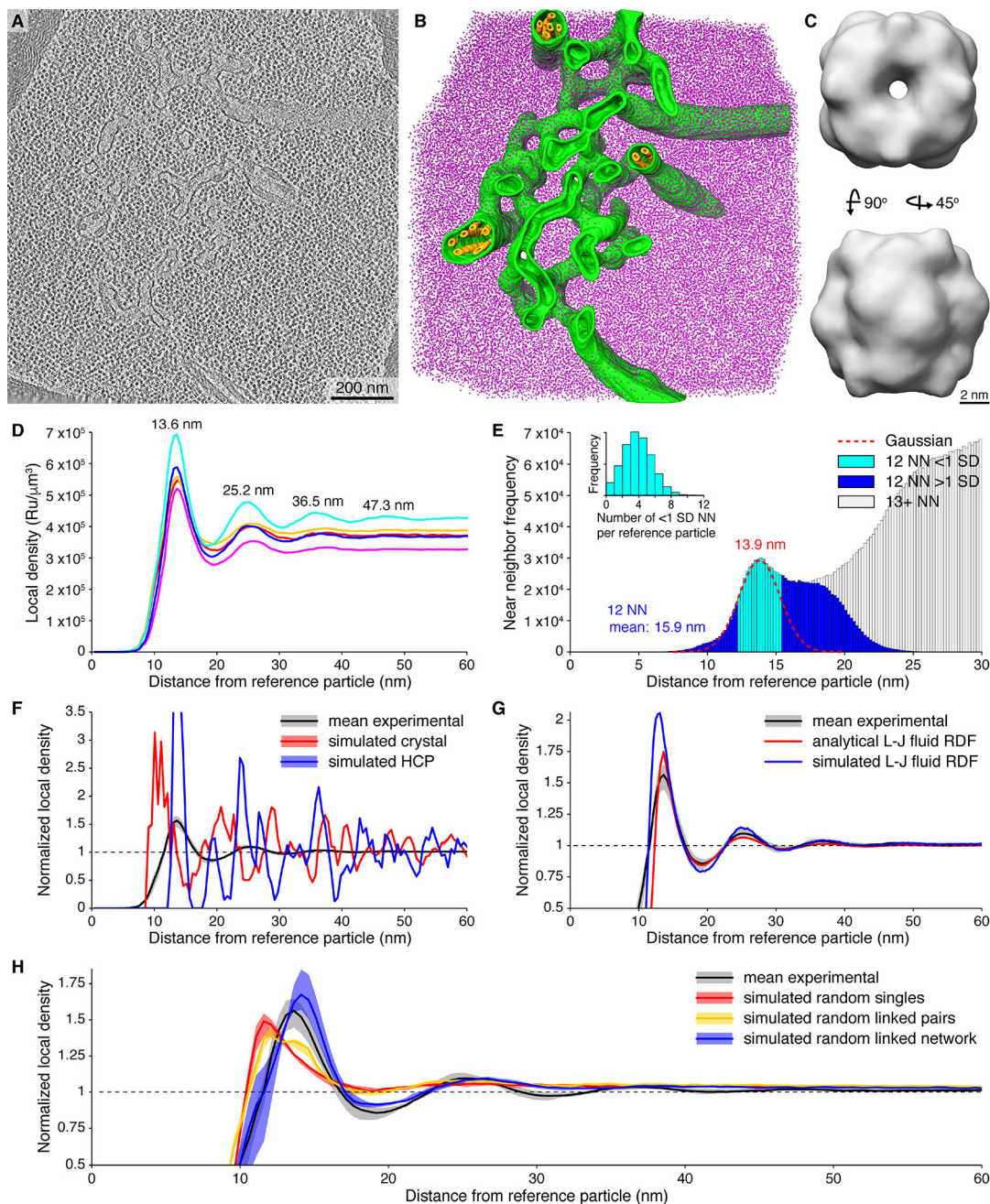
Figure 4. The Pyrenoid Matrix is not Crystalline but Exhibits Short-Range Liquid-Like Order
