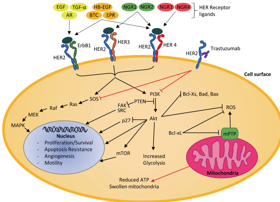
Fig. 1. Cellular response to HER/ErbB receptors dimerisation. HER/ErbB family receptors are activated upon homo-/hetero-dimerisation. With exception of HER2, activation is dependent on ligands binding to the extracellular domain, which subsequently causes phosphorylation of the intracellular kinase domain (except for the absent kinase domain for HER3) and initiates downstream cascades via PI3K and MAPK. The resulting effects of this cascade include proliferation, repair and resistant mechanisms that enhance survival. Trastuzumab binds to the HER2 receptor which either causes passive endocytosis leading to HER2 degradation, or the tumour cell is destroyed via antibody-dependent cell-mediated cytotoxicity (ADCC). Because of its inhibition, pro-survival signalling is reduced through decreased activity in downstream pathways. Cytotoxicity mediated through this inhibition is caused by generation of ROS and mitochondria dysfunctions, as well as increase of proapoptotic Bcl-xS. These cellular disruptions led swollen mitochondria and ATP depleted stores.
