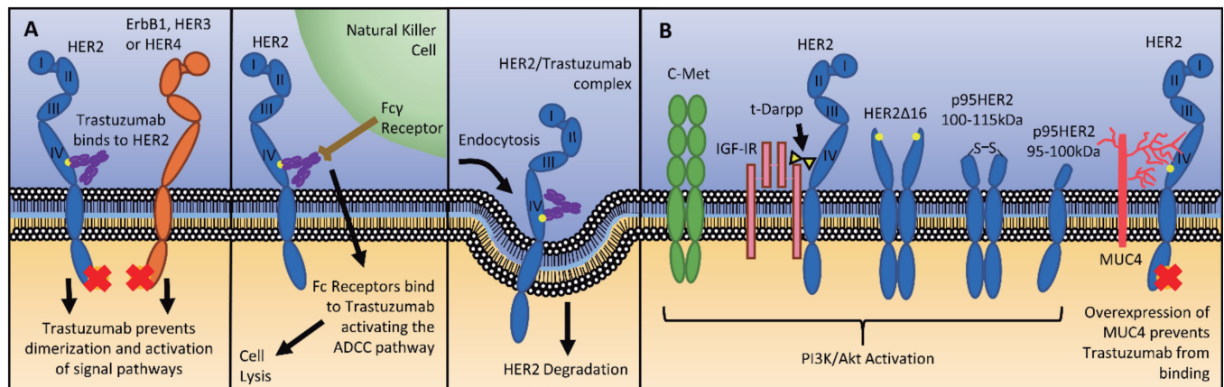
Fig. 2. Mechanisms of action and resistance for Trastuzumab. A. Trastuzumab binds to the extracellular domain blocking dimerisation of HER2 with other Her family members, thus preventing the activation of tyrosine kinase signalling pathways. Upon attachment of HER2, passive endocytosis takes place which causes HER2 degradation. The Fc region of Trastuzumab can attach to the Fc receptor of effector immune cells such as Natural Killer cells which destroys the tumour cell via antibody-dependent cell-mediated cytotoxicity (ADCC). B. In response to Trastuzumab, several biological alterations occur that help cells evade Trastuzumab treatment. Firstly, cells respond to treatment by rapidly upregulating C-Met and IGF-IR, where the former protects against Trastuzumab by abrogating p27 induction. Both activate downstream pathways normally sustained by HER2. IGF-IR signalling can also be activated through heterodimerisation with HER2 using t-Darpp which further increases resistance. Resistance can also arise from epitope masking from extracellular structures. Mucins, specifically MUC4 has been shown to play a role in the progression of cancer due to its anti-adhesive properties. In tumours, MUC4 can be overexpressed, presenting at the cell surface, where it is heavily glycosylated giving a highly extended and tough conformation. Its close association with HER2 helps mask Trastuzumab's target thereby offering protective resistance. Several isoforms of HER2 which are partly, if not all resistant to Trastuzumab exist; the most notable being HER2 \Delta 16 and p95HER2. HER2 \Delta 16 is formed by alternative splicing where it forms homodimers and constitutively activates downstream pathways. p95HER2 fragments can be formed from either alternative initiation of translation (100-115kDa) or proteolytic cleavage of HER2 by metalloproteases (95-100kDa). These fragments are hyperactive due to their ability to form dimers, and in the case of 100-115 kDa is maintained by disulphide bonds. The result are operational intracellular kinase domains, resistant to Trastuzumab.
