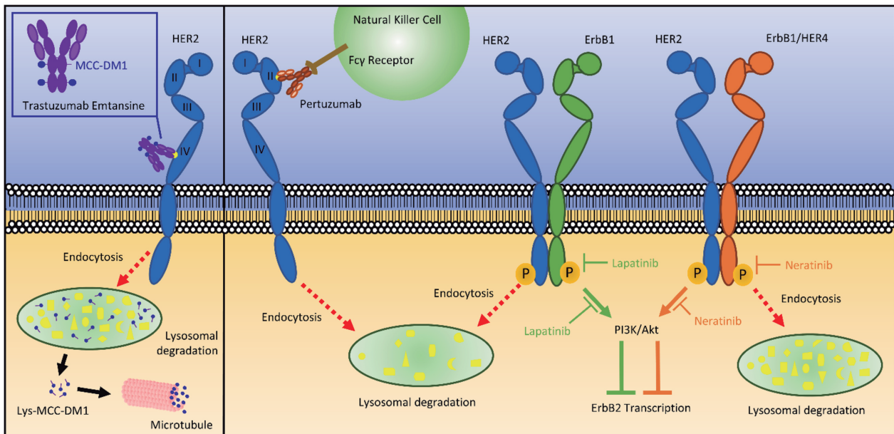
Fig. 3. Action sites of Trastuzumab Emtansine (T-DM1), Pertuzumab, Lapatinib and Neratinib. After attachment of Trastuzumab Emtansine to the extracellular domain IV of the HER2 receptor, the complex can either activate the antibody-dependent cellular cytotoxicity (ADCC) pathway (if an immune effector cell binds to the Fc region) or undergo endocytosis, whereby lysosomes degrade it. This releases DM1 metabolites which inhibits the assembly of microtubules by binding to tubulin and preventing cell division in tumour cells. Additionally, Trastuzumab binding to HER2 prevents both homodimerisation as well as HER2/HER3 heterodimerisation, which results in the inhibition of the PI3K and MAPK signalling cascades. This suppresses cellular proliferation and survival mechanisms that are fundamental to tumorigenesis. Similarly, Pertuzumab can also activate the ADCC pathway or cause endocytosis, although it attaches to extracellular domain II. Both small molecule inhibitors, Lapatinib and Neratinib, target the intracellular domain activity of the HER2 receptor. These work by blocking the downstream PI3K/Akt pathways, which regulates ErbB2 transcription. In the presence of either of these drugs, the drug-receptor complex undergoes passive endocytosis and lysosomal degradation. Neratinib can also trigger potent ubiquitination and vigorous degradation, whereas Lapatinib has stronger suppressive effects on ErbB2 transcription.
