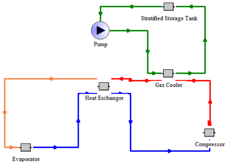
Figure 1: The schematic diagram of the heat pump water loop.
