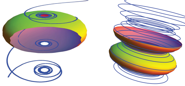
Figure 1: Two magnetic trajectories obtained as images by \mathcal{H}_0 of two free elasticae. According to Theorem 1, they lie into two surfaces of revolution (shown in part) on which they have been chosen to have the same Clairaut slope.
