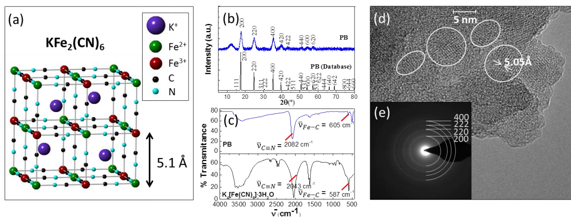
Figure ¡Error! solo el documento principal.. a) PB structure b) XRD patterns of the PB synthesized and the PB listed in ICSD Karlsruhe Database (n° 162081). 39 The Kapton ® film peak has been marked with an *. c) IR spectra of PB and the starting reagent, K_4[Fe(CN)_6] \cdot 3H_2O , labelling the characteristic C \equiv N and Fe-C \equiv N absorption bands of both. d) TEM image of PB domains and e) electron diffraction pattern of PB nanocrystals with crystallographic planes indexed.
