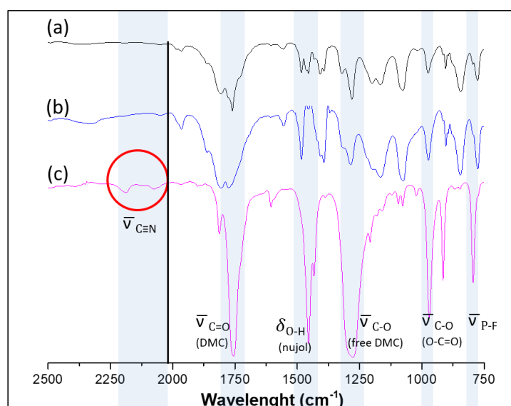
Figure 6. FTIR spectra of a.) the electrolyte ( \text{LiPF}_6 1M EC:DMC), b.) the electrolyte in contact with PB and c.) the glass fibre of a fully discharged battery washed with DMC.
