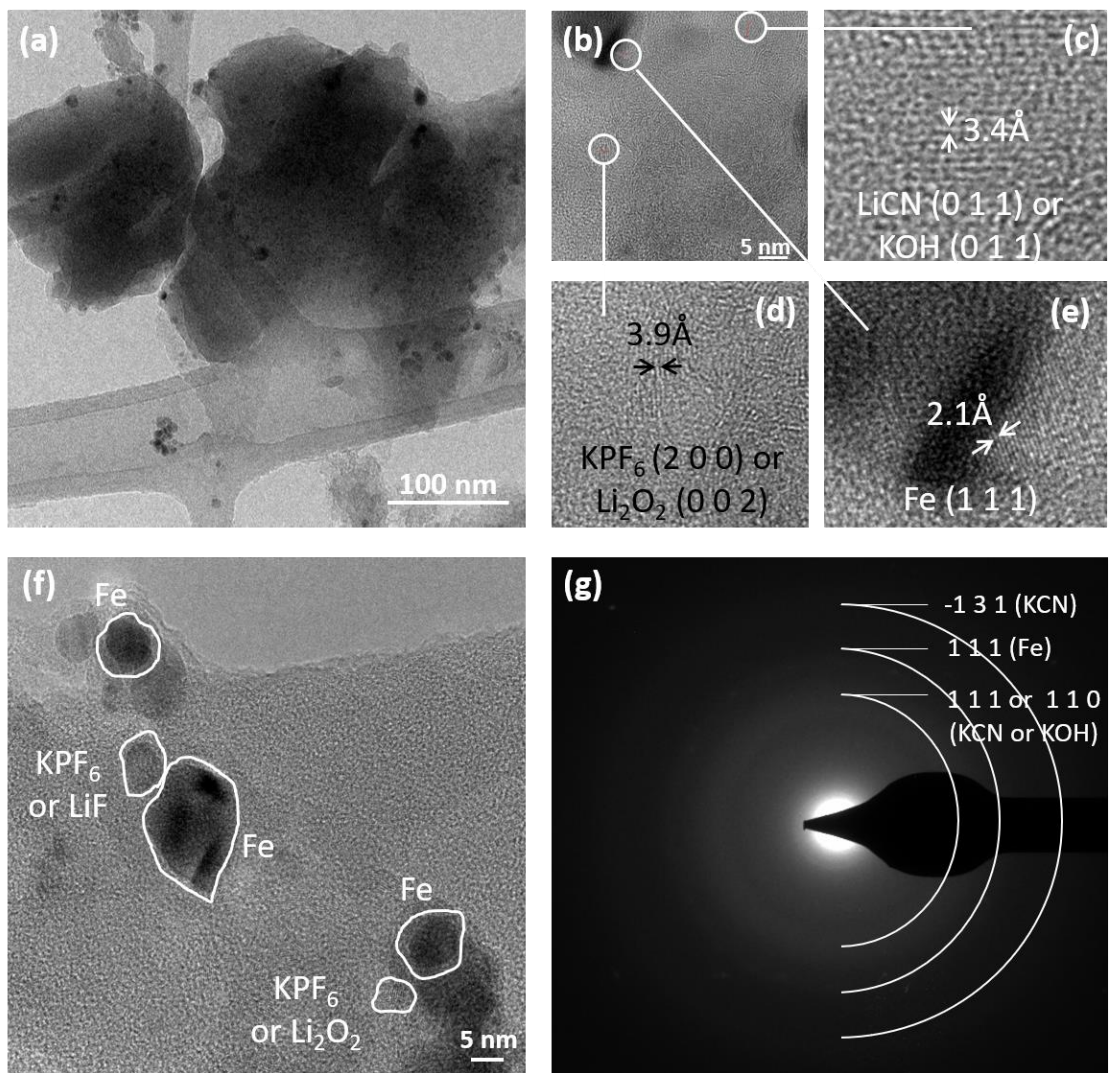
Figure 8. a.) TEM image of the material from a fully discharged half battery. b.) TEM image of a completely discharged battery displaying several domains and their higher magnification (c, d and e). f.) Different domains observed in a completely discharged battery, possibly containing Fe, LiF and KPF 6 . g) Electron diffraction pattern of another area of the same fully discharged battery. White lines schematically indicate the broad diffraction rings with the crystallographic planes of possible reaction compounds.
