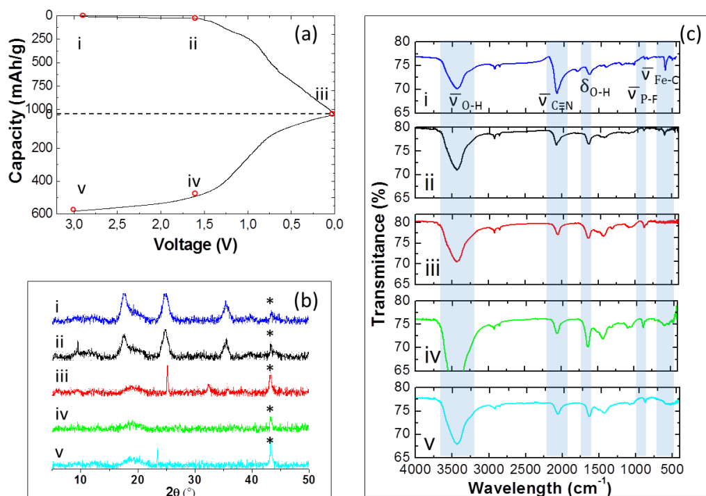
Figure 5. a) First discharge and charge profile of PB/Li cell at R.T. in a voltage range of 0.005-3.2 V. b) XR diffractograms of the electrodes in the different points (i, ii, iii, iv, v) of the galvanostatic curve of Fig.5a. The reflections due to the Cu-foil are marked with an *. c) IR spectra of the electrodes in the different points (i, ii, iii, iv, v) of the galvanostatic curve (Fig.5a).
