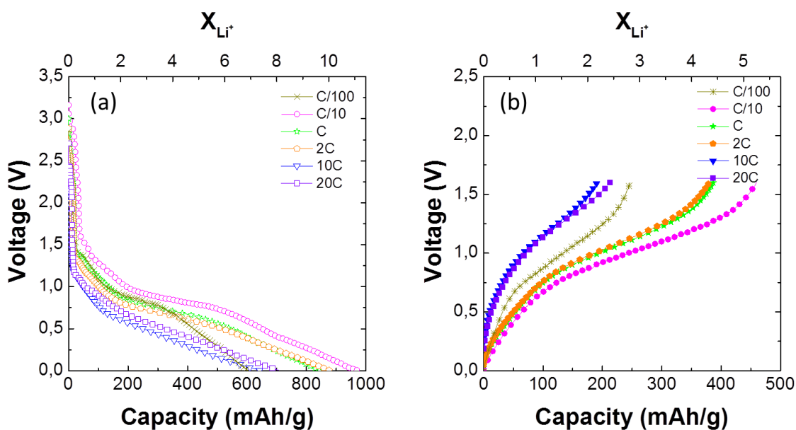
Figure 3 Galvanostatic first discharge (a) and first charge (b) curves of PB/Li cells measured at different currents (from C/100=0.875 mA·g -1 to 20C = 1.750 A·g -1 ) in the voltage range 0.005-1.6 V.
