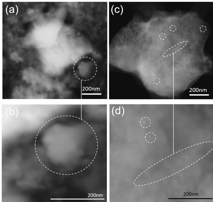
Figure 7. SEM-STEM images of the pristine material (a) the material completely discharged (c) and zoomed zones of both of them, respectively (b,d).
