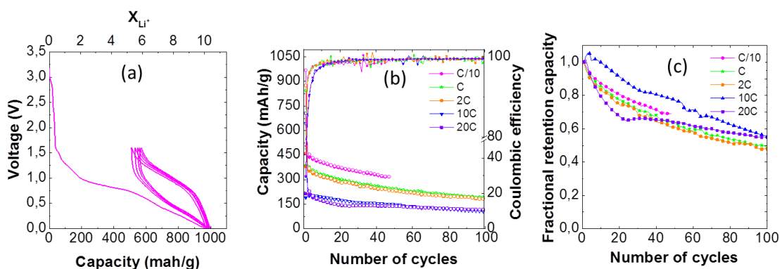
Figure 4. Electrochemical performance of PB when tested vs lithium with LiPF 6 in EC:DMC. a) Voltage profile during the five first cycles of galvanostatic discharge and charge at C/10. b) Specific capacity of PB at different C-rates and their coulombic efficiency. c) Capacity retention vs cycle number for different C-rates.
