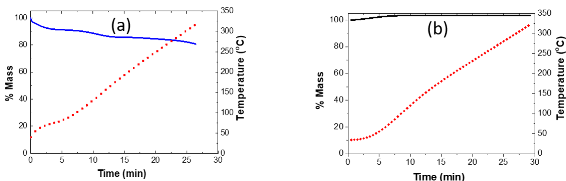
Figure ¡Error! solo el documento principal.. Thermogravimetric analysis of pristine PB (a) and Prussian White (b), scanned from 30 to 325°C using N_2 atmosphere and a temperature step of 10 K/min.
