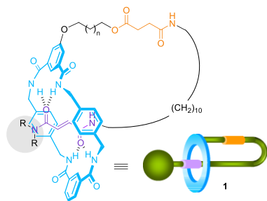
Fig. 1 Bistable [1]rotaxanes 1 and its schematic representation.
