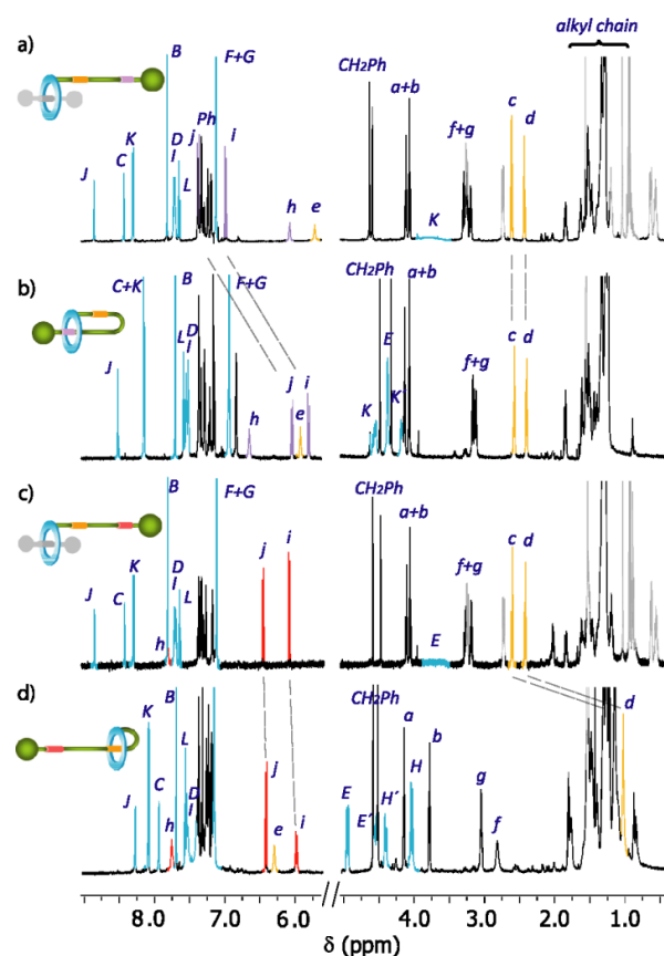
Fig. 5 Partial 1 H NMR spectra (600 MHz, CD_2Cl_2 , 298 K) of (a) succ - E - 10 , (b) [1]rotaxane E - 1c , (c) succ - Z - 10 and (d) [1]rotaxane Z - 1c . Peaks corresponding to the N,N,N',N' -tetrabutylsuccinamide component in succ - E - 10 and succ - Z - 10 are in grey. Lettering is shown in Schemes 2 and 3.
