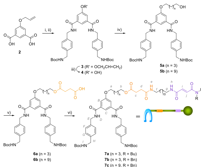
Scheme 1 Synthesis of the U-shaped precursors 7 . Reagent and conditions: i) (COCl) 2 , DMF (dimethylformamide) cat., CH 2 Cl 2 , reflux; ii) H 2 NCH 2 C 6 H 4 CH 2 NHBoc, Et 3 N, CH 2 Cl 2 , 0-25 °C, 93% (two steps); iii) Pd(PPh 3 ) 4 , NaBH 4 , THF (tetrahydrofuran), rt, 96%; iv) Br(CH 2 ) n+2 OH (n = 3 or 9), NaI, K 2 CO 3 , (CH 3 ) 2 CO, reflux, 5a (n=3), 70%; 5b (n=9), 93%; v) succinic anhydride, DMAP (dimethylaminopyridine), THF, reflux, 6a (n=3), 80%; 6b (n=9), 97%; vi) (E)-R 2 NCOCH=CHCONH(CH 2 ) 12 NH 2 ( S1a , R = Bu or S1b , R = Bn), Castro's reagent: BOP (benzotriazol-1-yloxytris(dimethylamino)phosphonium hexafluorophosphate), Et 3 N, CH 2 Cl 2 , rt, 7a (n=3, R = Bu), 82%; 7b (n = 3, R = Bn), 67%; 7c (n = 9, R = Bn), 78%. Full experimental procedures can be found in the ESI†.
