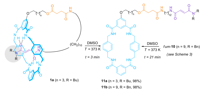
Scheme 4 Dethreading of the [1]rotaxane 1a and the [2]rotaxane fum-10 .
