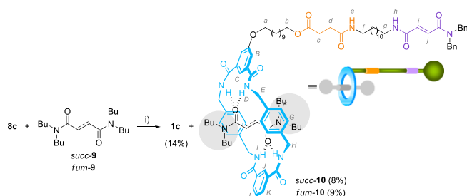
Scheme 3 Competitive coupling of the diamine 8c with isophthaloyl chloride in the presence of single binding-site threads: formation of the [1]rotaxane 1c using an intramolecular template versus the formation of [2]rotaxanes 10 using the intermolecular dicarboxamide-based templates 9 . Reagent and conditions: i) isophthaloyl chloride, Et 3 N, CHCl 3 , 25 °C.
