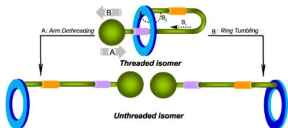
Fig. 4 Unthreading mechanisms of a (pseudo)[1]rotaxane with a ring having two different faces (in dark and light blue). Note that a ring tumbling of the threaded isomer inverts the face of macrocycle during the exchange to the unthreaded isomer. Also for clarity, sequential motions B1 and B2 of the ring tumbling process B are also indicated (dashed arrows).
