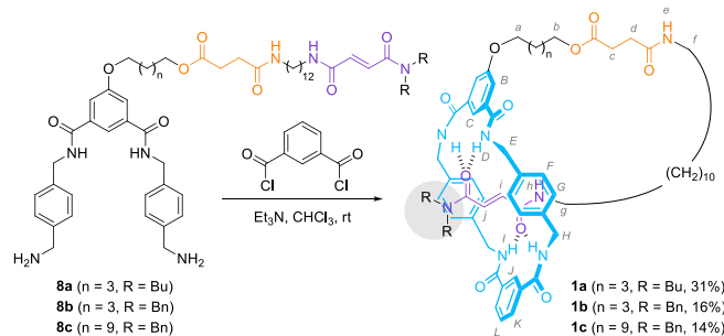
Scheme 2 Synthesis of benzylic isophthalamide macrocycle-based (pseudo)[1]rotaxanes 1 .
