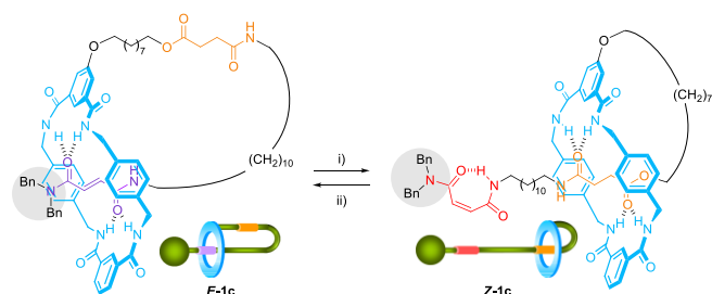
Scheme 5 Light-driven exchange of the extended and contracted forms, E - 1c and Z - 1c , of the benzylic isophthlamide [1]rotaxane. Conditions: i) 254 nm (62 W·m -2 ), CH_2Cl_2 , 90 min, 51%; ii) 312 nm (56 W·m -2 ), CH_2Cl_2 , 35 min, 95%.
