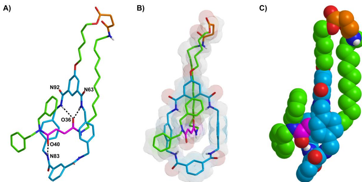
Fig. 3 X-Ray structure of the benzylic isophthalamide [1]rotaxane 1b . A) Side-on view of a capped-sticks model of 1b displaying the interaction between the ring and the fumaramide binding site. B) Front view of stick and CPK model of 1b showing the threading of the arm. C) Peripheral view of a space-filling model of 1b enlightening its extended lasso conformation. For clarity, non-polar hydrogen atoms, solvent molecules and disorder have been omitted ( C_{\text{macrocycle}} , light blue; C_{\text{arm}} , green; C_{\text{fumaramide}} , purple; C_{\text{succinamide}} , orange; O, red; N, blue; H, white). Intramolecular hydrogen-bond lengths [Å] (and angles [deg]): O36HN63 2.400 (177.9); O36HN92 2.220 (171.3); O40HN83 2.054 (179.4).
