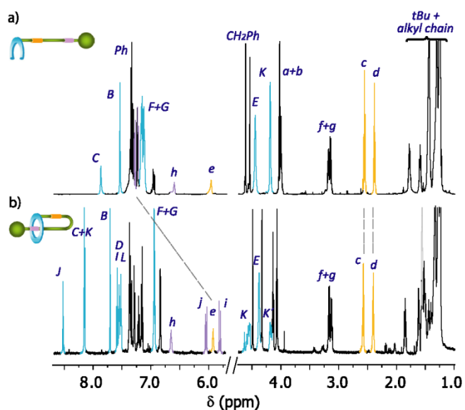
Fig. 2 Partial ^1\text{H} NMR spectra (600 MHz, \text{CD}_2\text{Cl}_2 , 298 K) of (a) precursor 7c and (b) [1]rotaxane 1c . The assignments correspond to the lettering shown in Schemes 1 and 2.
