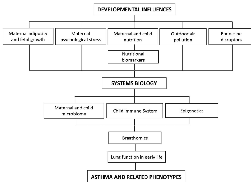
FIGURE 3 Diagram of the different research areas covered by the nutrition in early life and asthma (NELA) cohort and their interactions
